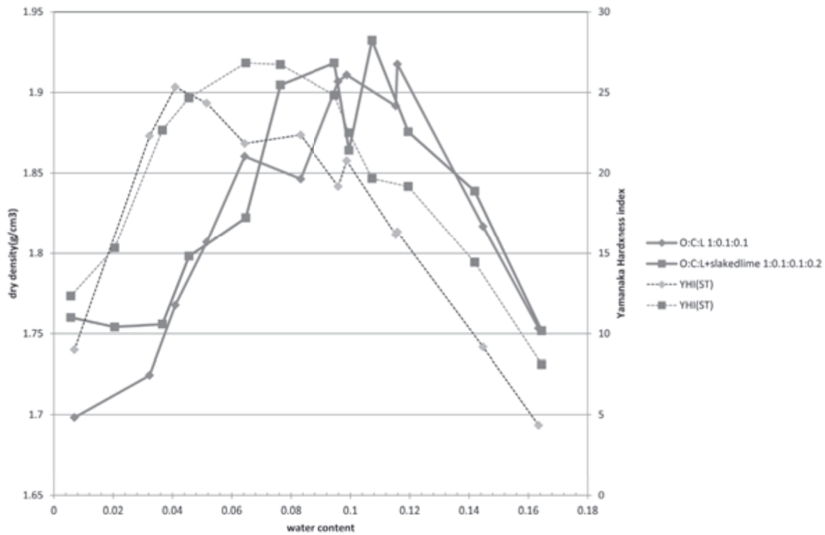
Fig. 10: Compaction test
