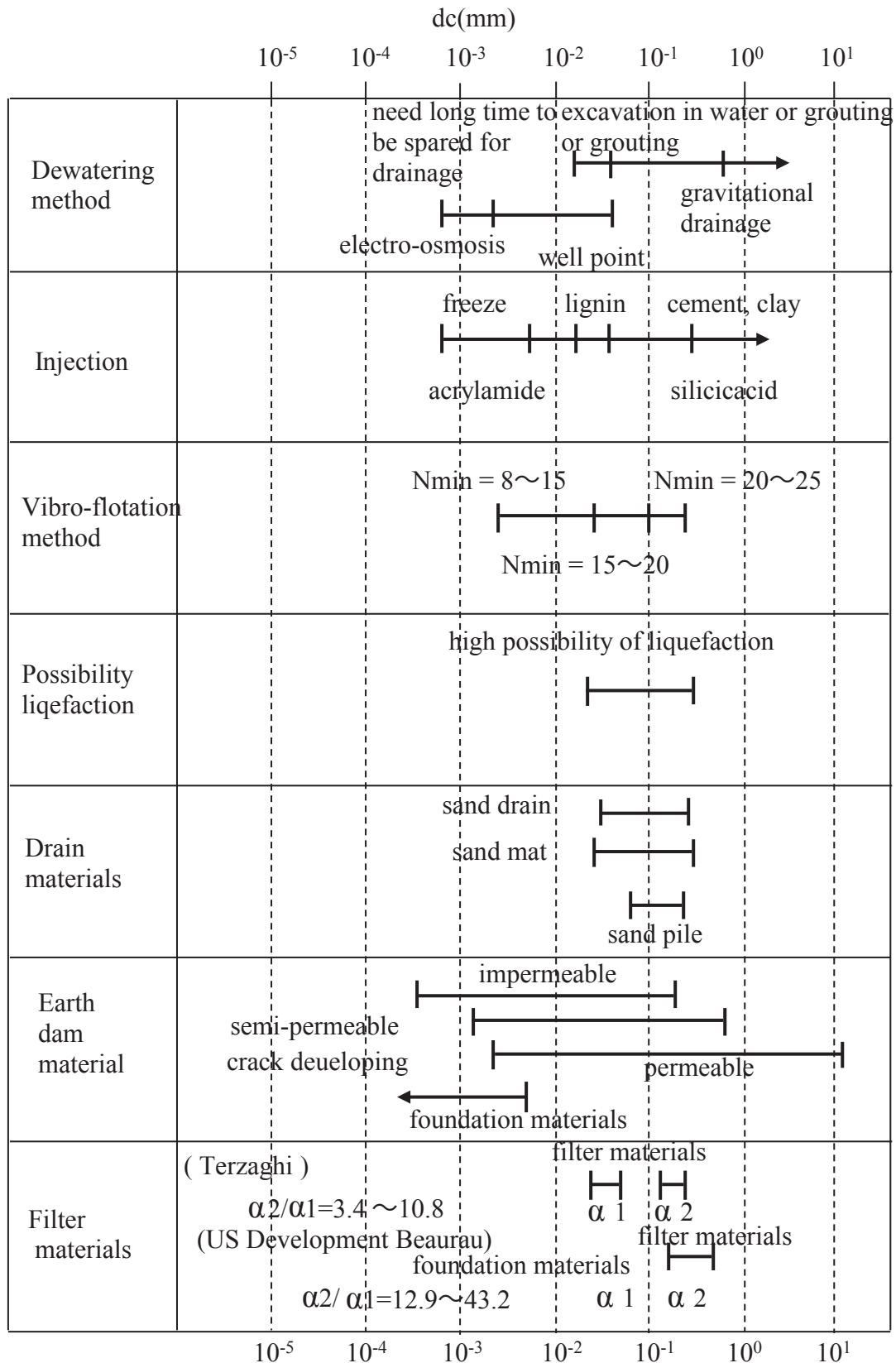
Fig. 6: Representative diameters and soil properties
