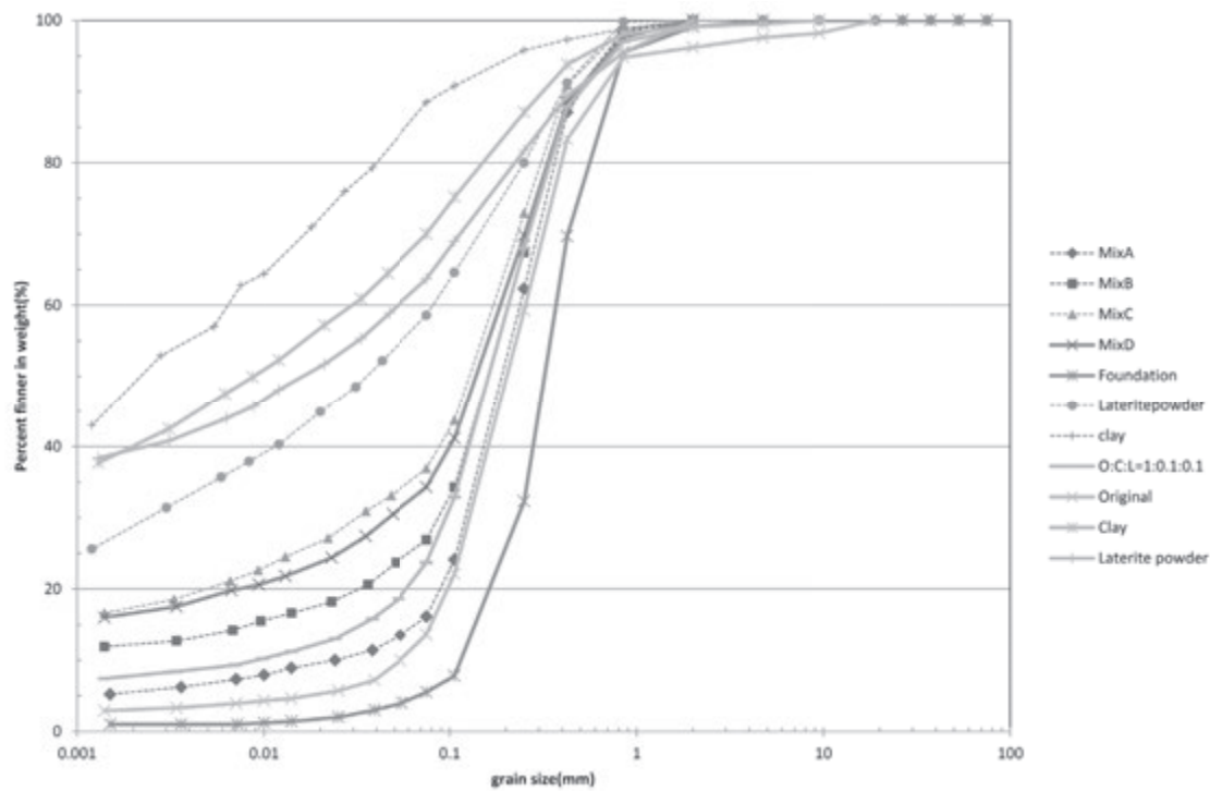
Fig. 13 : Consolidation of the coarse excavated sand by mixing clay
