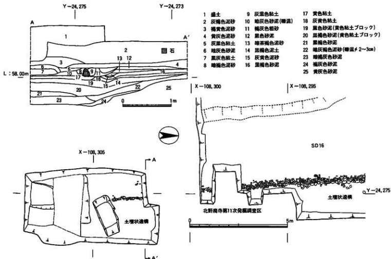
図21 遺構実測図 (1/40, 1/100)
