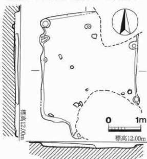
Fig.12 S I 1 5 0 (1/80)
