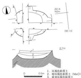
図29 SKc7 (S=1/30)
