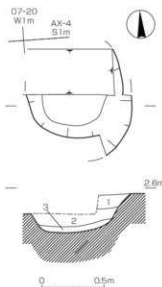
図19 SKb1 (S=1/30)
