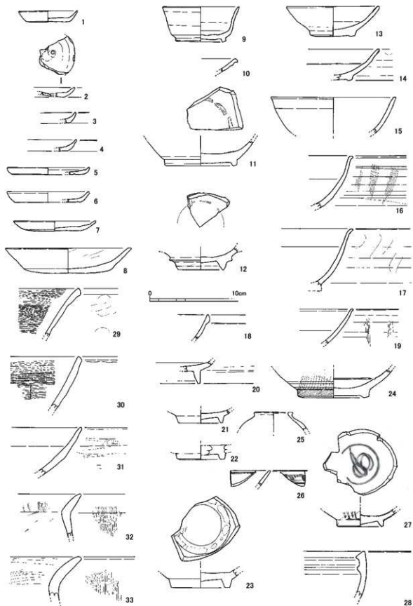
Fig.183 邛区235号遺構出土遺物実測図1(1/3)
