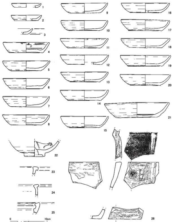
Fig.185 Ⅱ区320号遺構出土遺物実測図(1/3)
