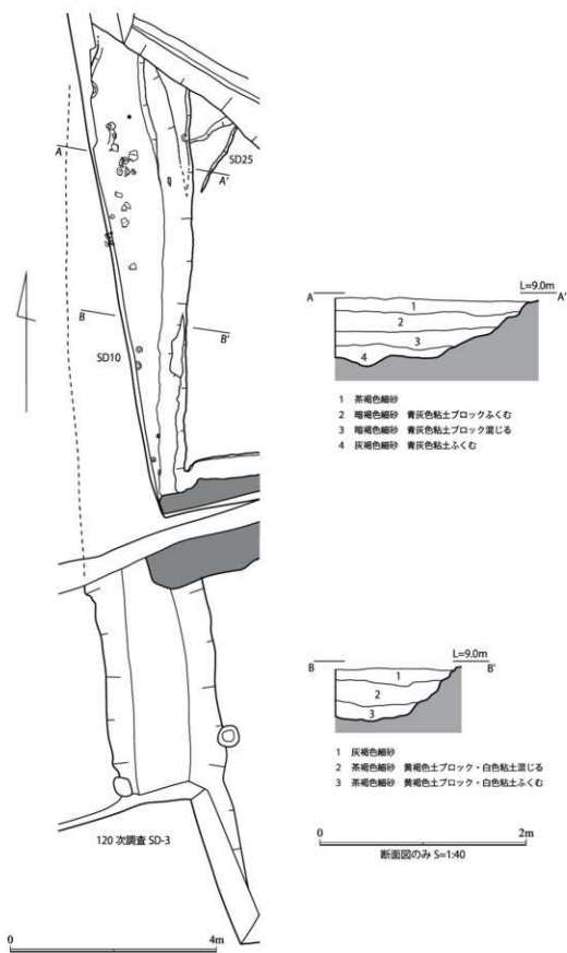
図8 SD10 (S=1/80)
