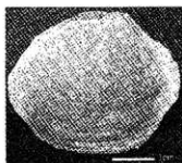
38. Macoma optiva (Yokoyama) 掘削岩塊 MORI-05080901
