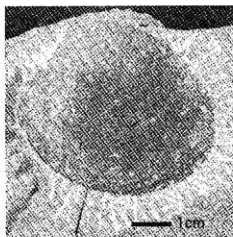
43. Pitar matsumotoi (Nagao) 掘削岩塊 OTA-05082517
