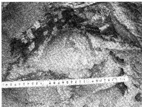
30. Chlamys ashiyaensis Bed C区画 Loc.7 OTA-05080805
