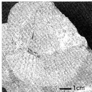
32. Fragments of Chlamys sp. 掘削岩塊 OTA-05080807
