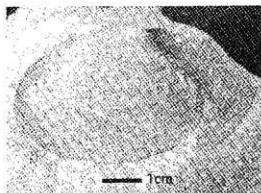
42. Pitar ashhyaensis (Nagao) 掘削岩塊 OTA-05082516
