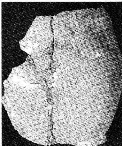
31. Chlamys ashhyaensis (Nagao) within Chlamys ashhyaensis Bed C区画 Loc.7 OTA-05080805
