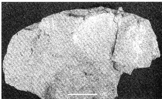
31. Block of sandstone with Chlamys sp. and Yoldia sp.
