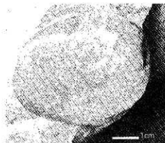
44. Pitar sp. 掘削岩塊 OTA-05082518
