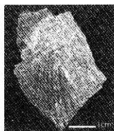
32. Fragment of Chlamys sp. 掘削岩塊 OTA-05080806
