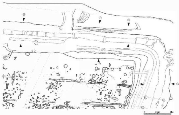
21SD1 断面⑧ W 10+23.0m
