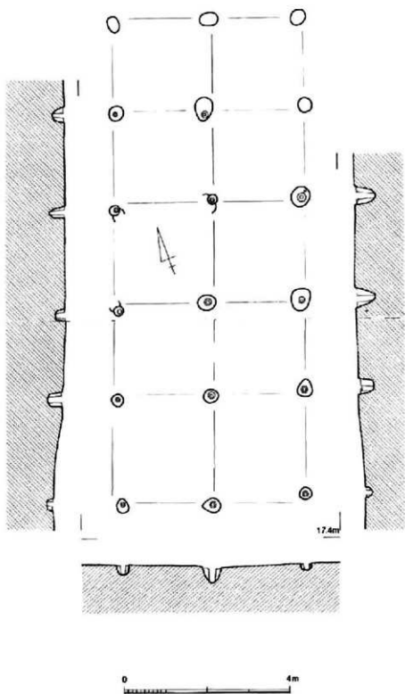
掘立柱建物20 (SB80045)
