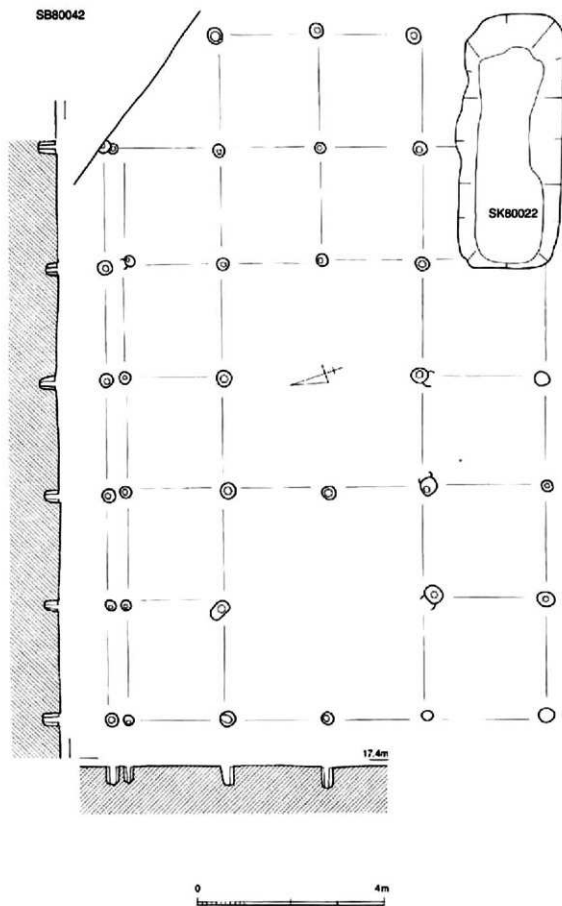
獨立柱建物17 (SB80042)
