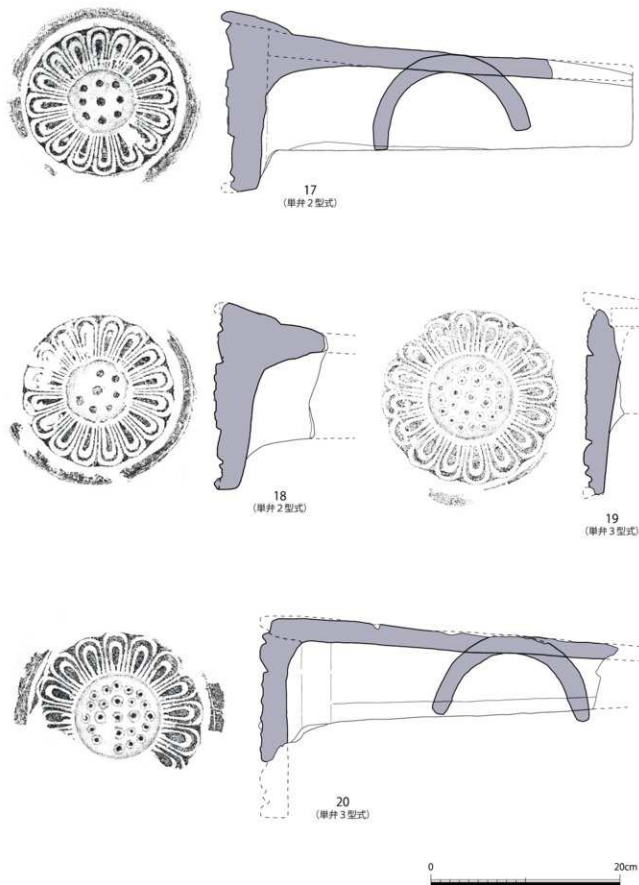
图26 軒丸瓦実測図 (1/4)
