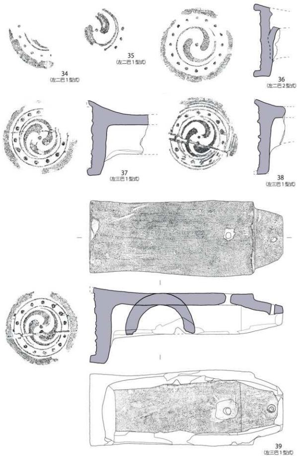
图26 軒丸瓦実測図 (1/4)
