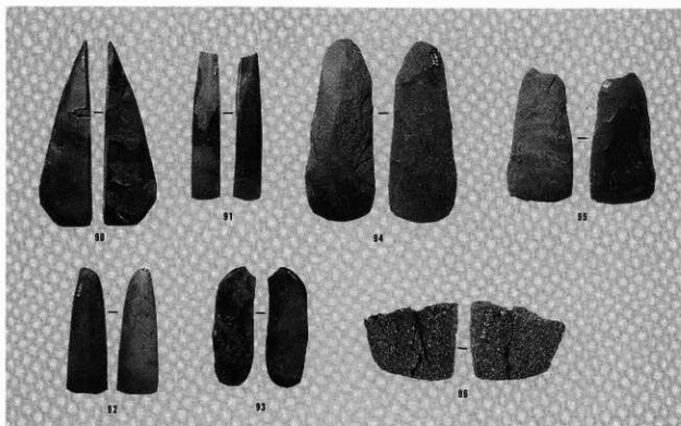
1 P-2の遺物(2) (1/3)
