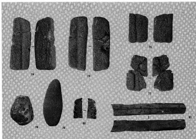
1 P-28の遺物(3) (1/3)
