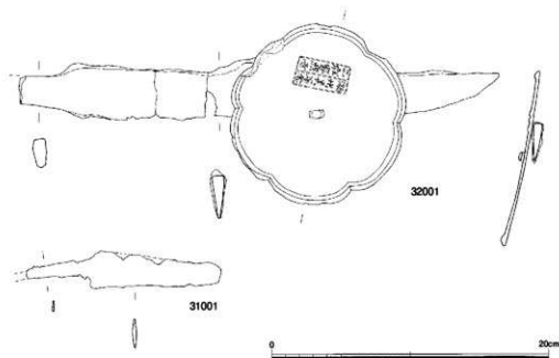
Fig.68 SR8014出土遺物実測図1(1/3)
