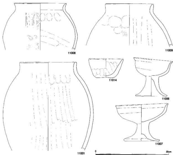
Fig.44 SC4007出土遺物実測図2(1/3)
