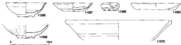
Fig.62 SC8001出土遺物実測図(1/3)
