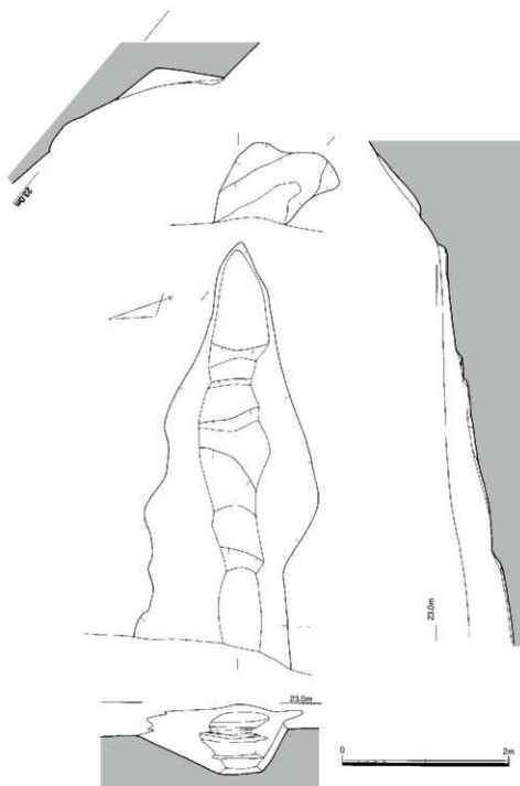
Fig.87 SX9002遺構実測図(1/50)
