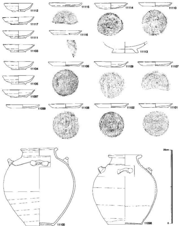
Fig.69 SR8014出土遺物実測図2(1/3)
