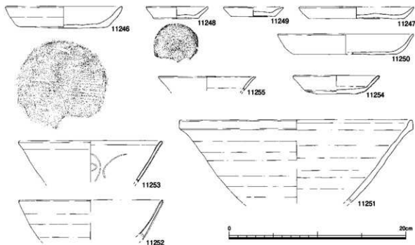
Fig.96 10区出土遺物実測図(1/3)
