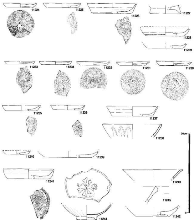
Fig.94 10区出土遺物実測図(1/3)
