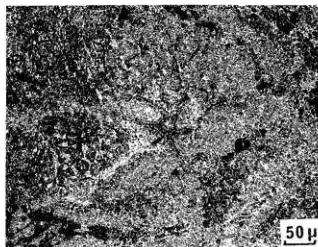
ひも状黒鉛
