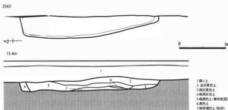
Fig.3 2SI01 遺構実測図 (1/40)
