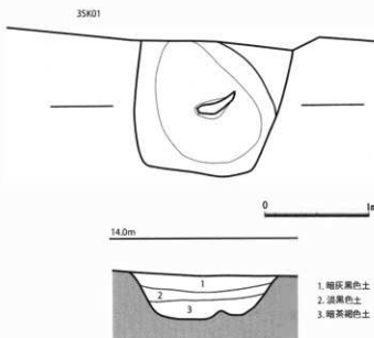
Fig.8 3SK01 遺構実測図 (1/40)
