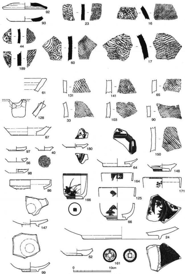
Fig.8 遺物実測図 S = 1 : 3
