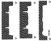
SB1260
