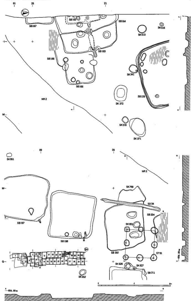
図版38 遺構実測図26
