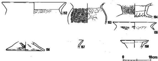
図12 遺構出土遺物実測図5 (S=1/4)
