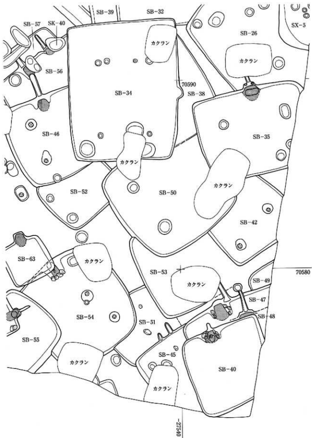
図14 下層遺構実測図⑤ (1:100)
