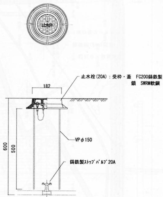
止水栓
