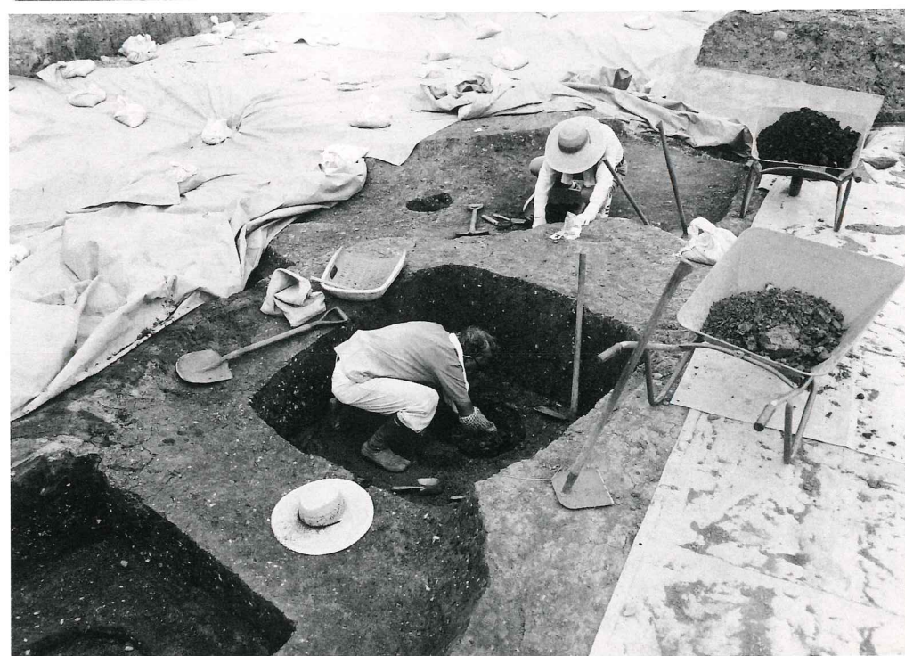
(3) 調査風景 (SH5の大型掘立柱建物の調査風景)
