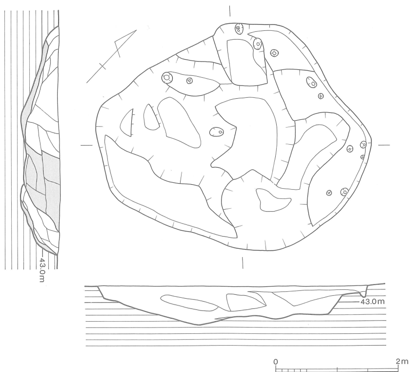
Fig.10 SX12実測図 (1/60)
