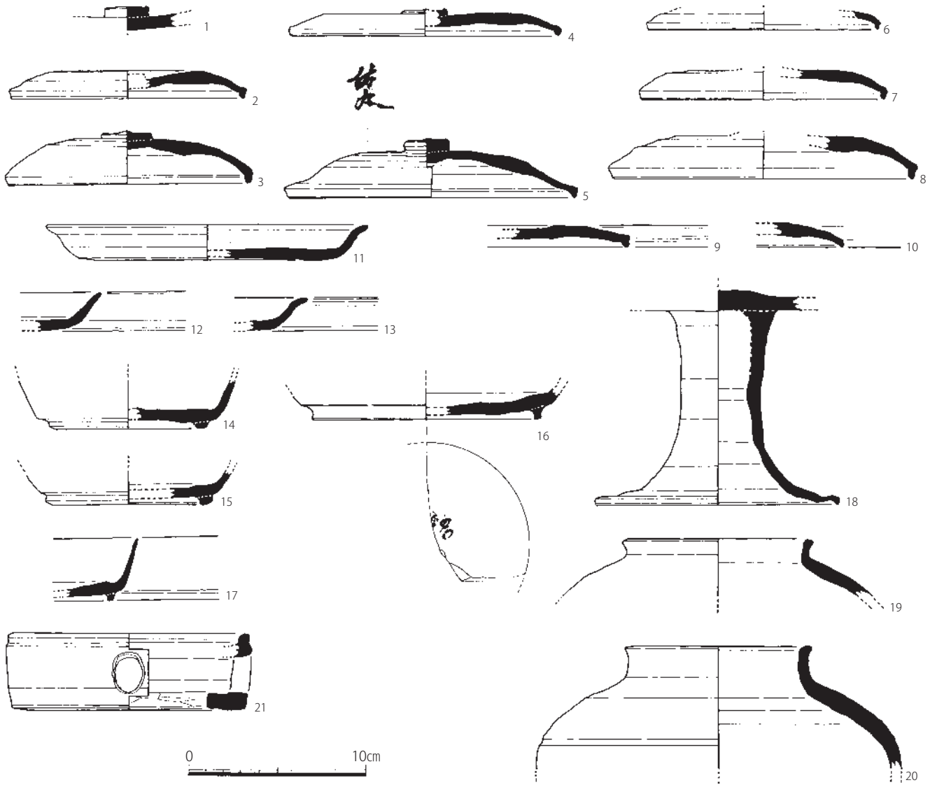
Fig.6 38SD001 灰色粘土出土遺物実測図 (1/3)
