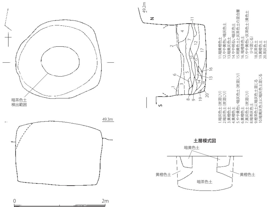
Fig. 171 294SK001 遺構実測図 (1/40)
