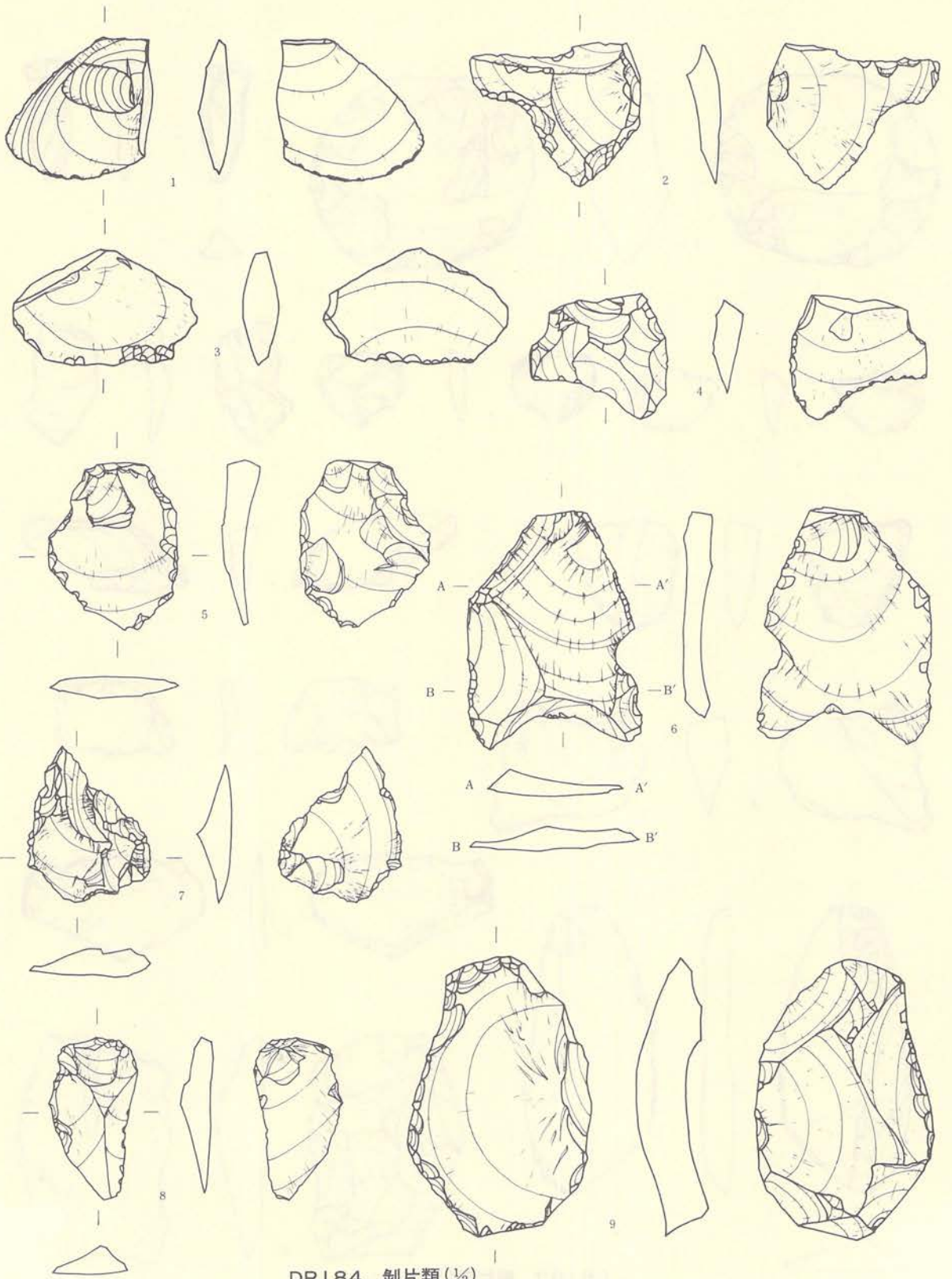
DR184 剥片類(1/2)
