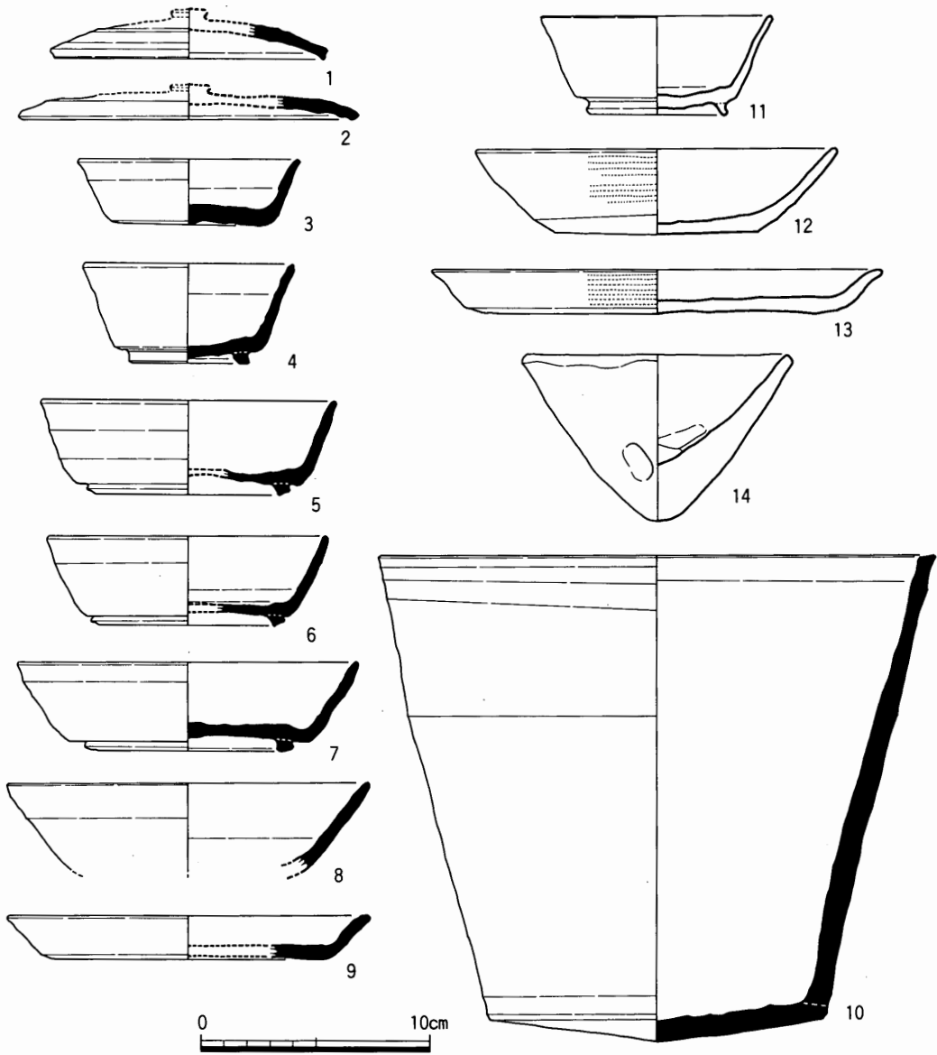
Fig.112 89SK115出土遺物実測図(1/3)
