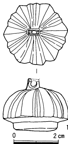
Fig.130 暗黒茶色土出土遺物実測図(2)(1/1)
