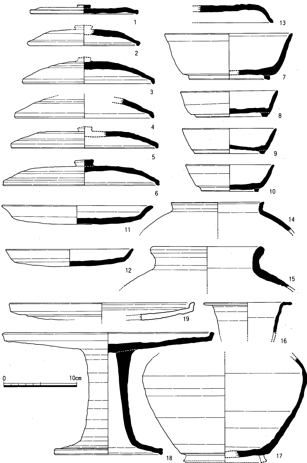
Fig. 100 89SK020出土遺物実測図(1)(1/3)
