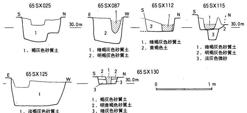
Fig.16 掘り方状遺構土層観察図(1/40)
