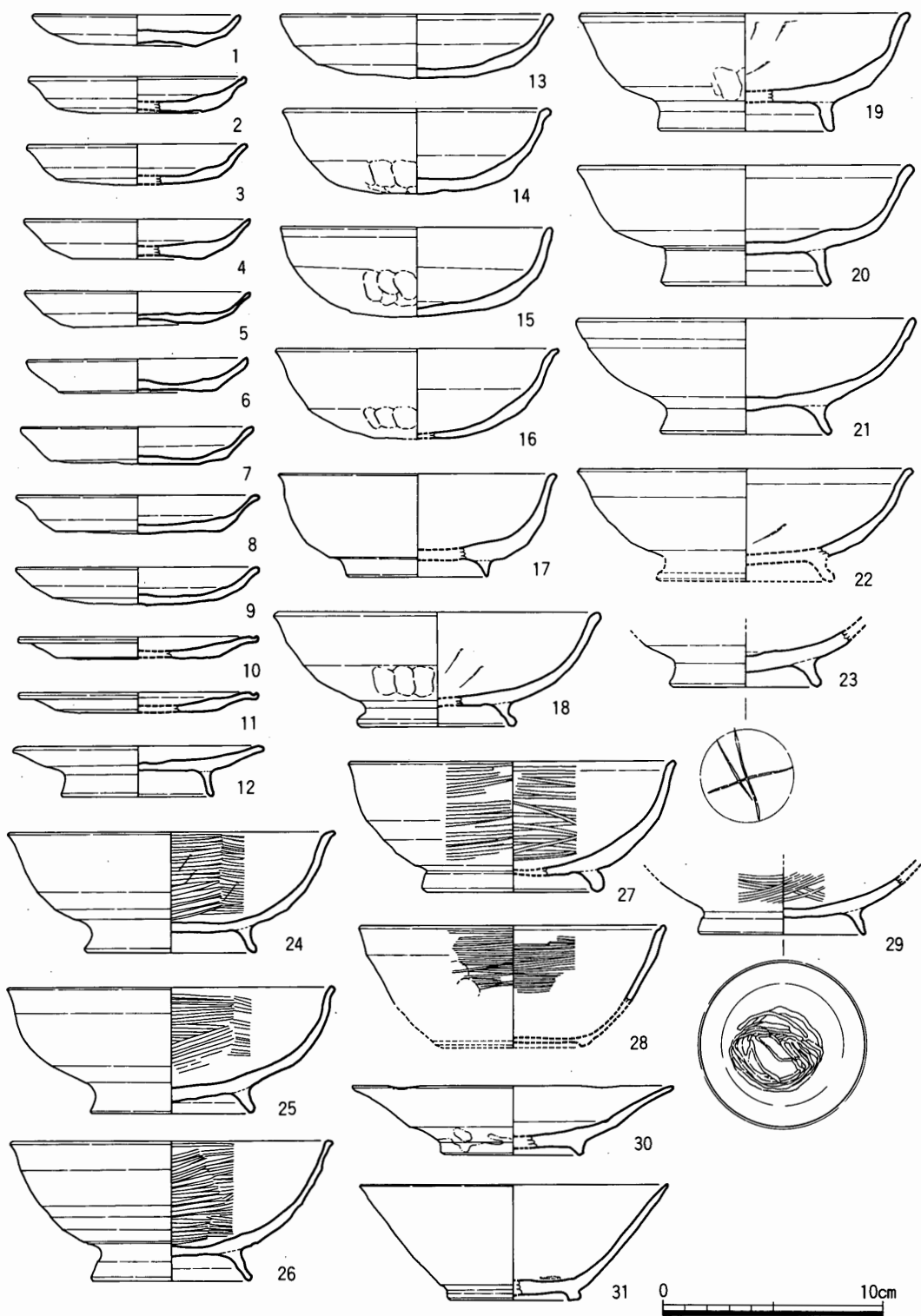
Fig. 104 89SK050出土遺物実測図(1)(1/3)
