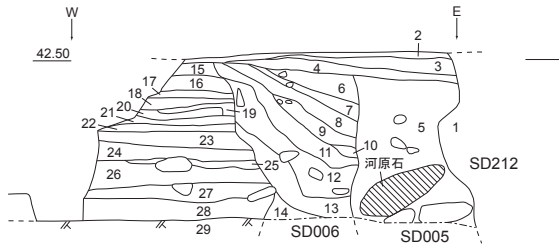
3-4-27 SD005 断面図②(1/30)
