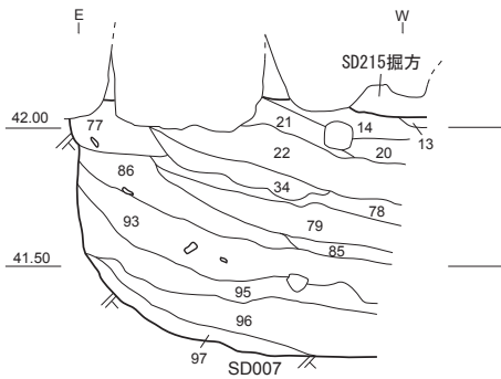
5-1-05 SD007 断面図③(1/30)
