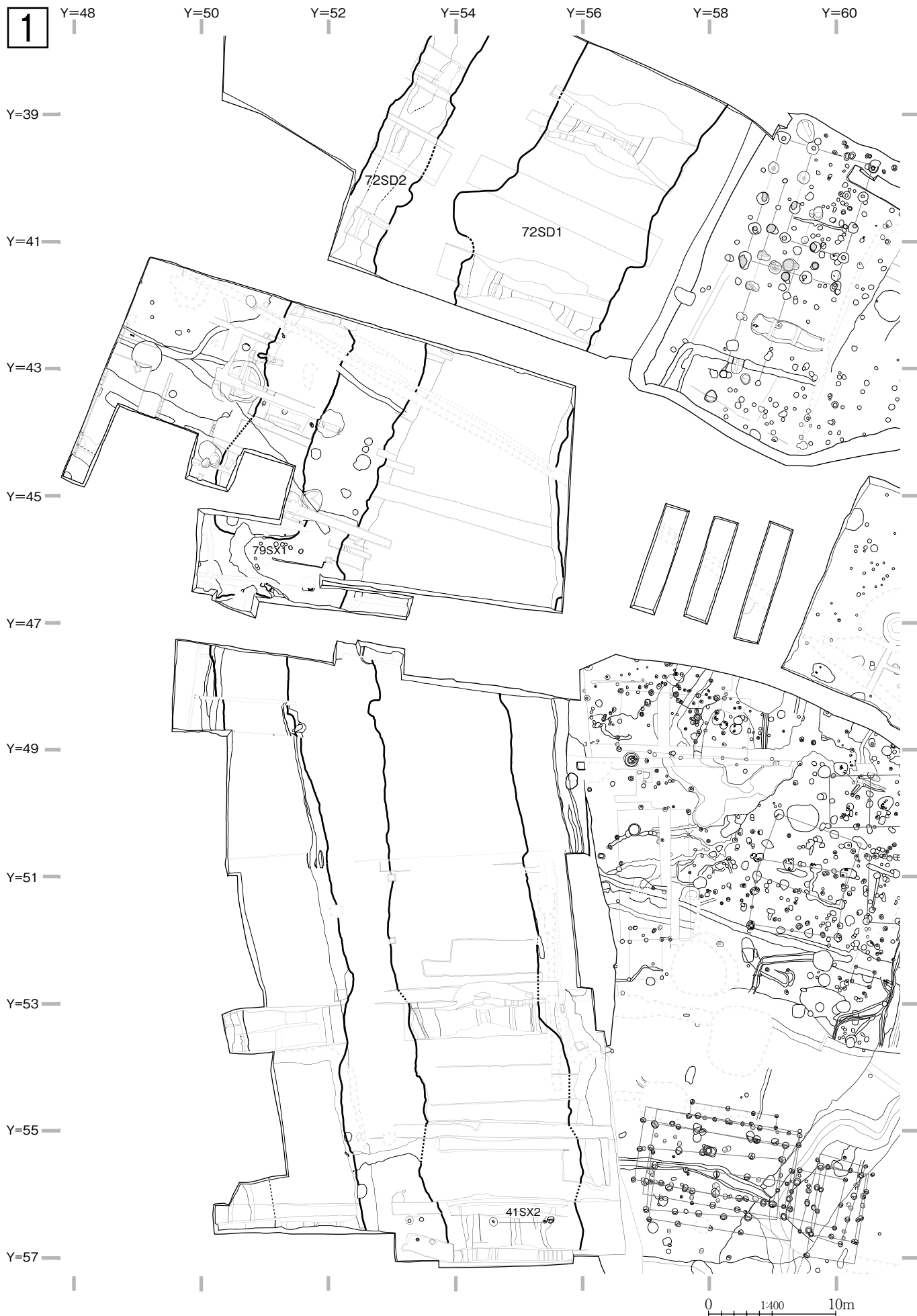
图74 掘跡① (72SD1·72SD2)
