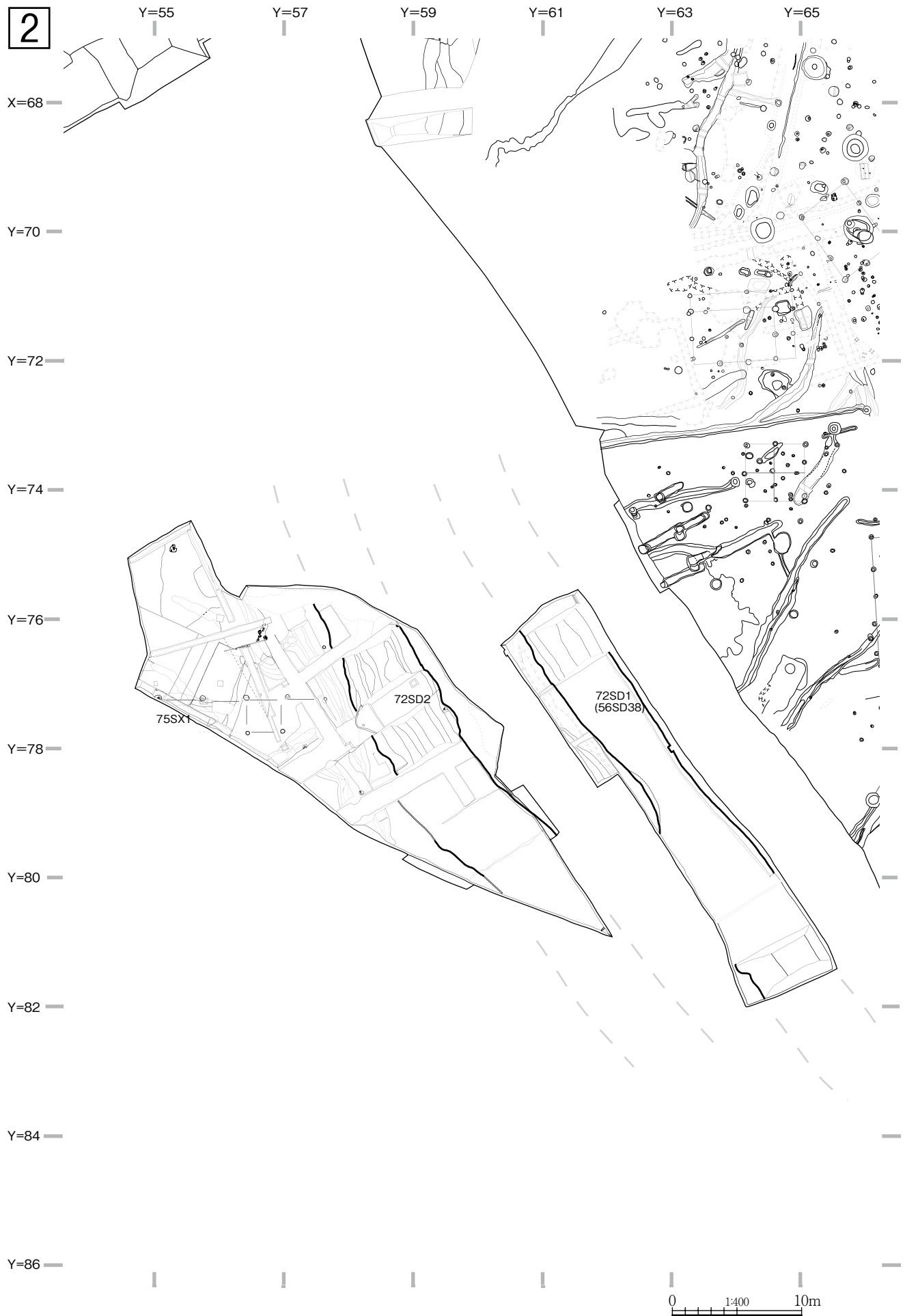
图75 掘迹② (72SD1·72SD2)
