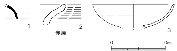
図15 SK6出土遺物実測図(1/4)
