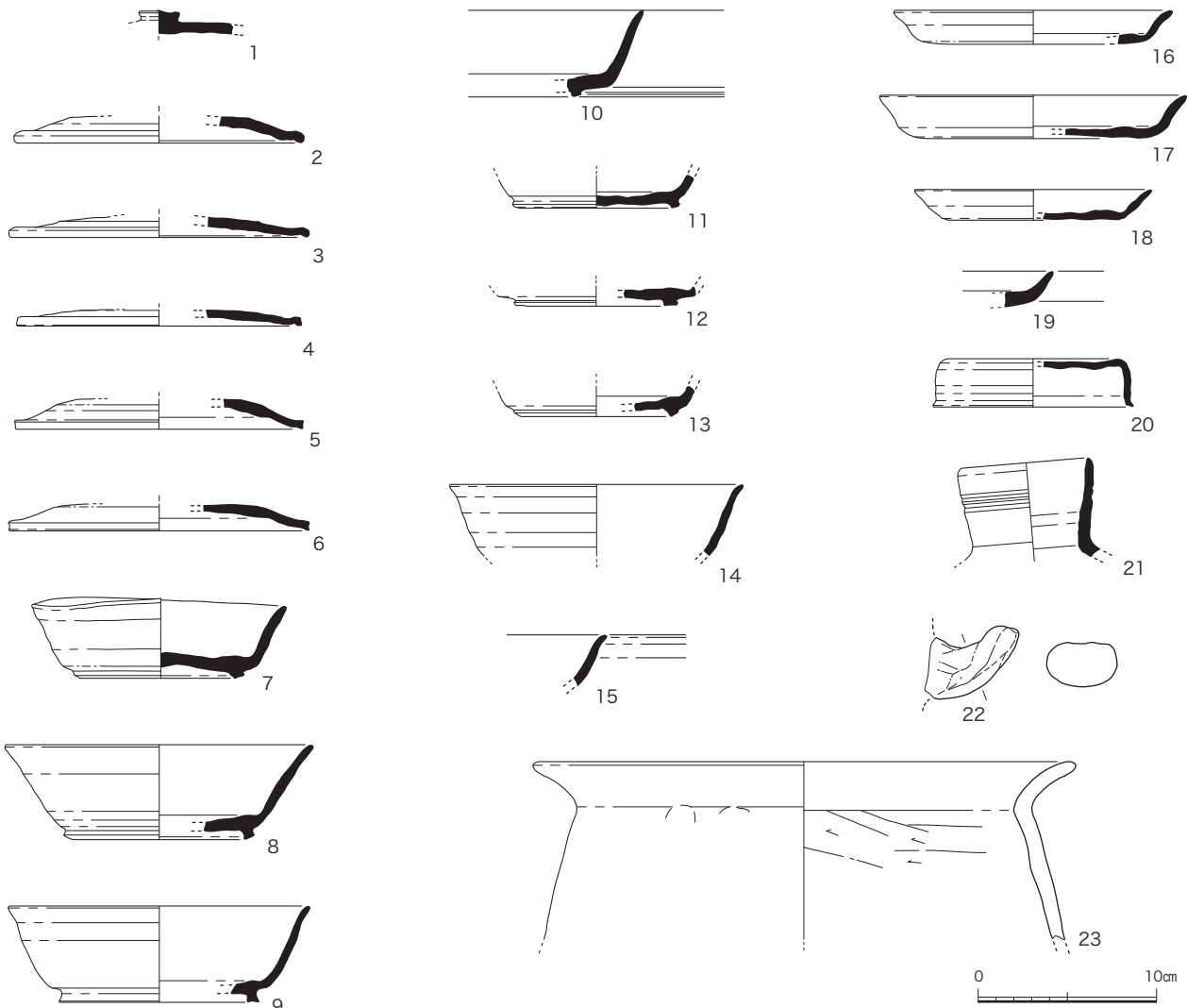
図10 SK4出土遺物実測図(1/4)
