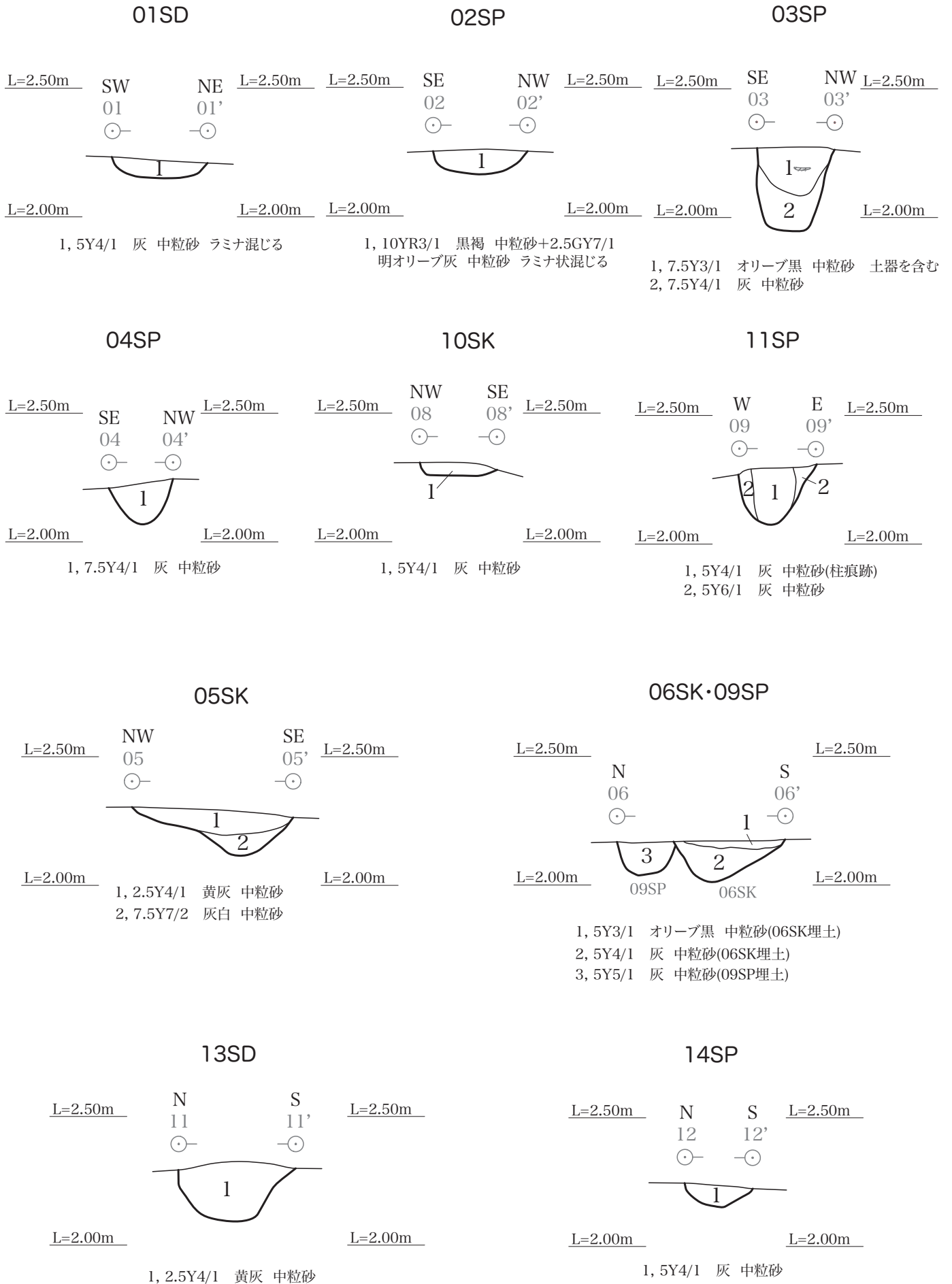
図6 個別遺構図-2 (1:20)
