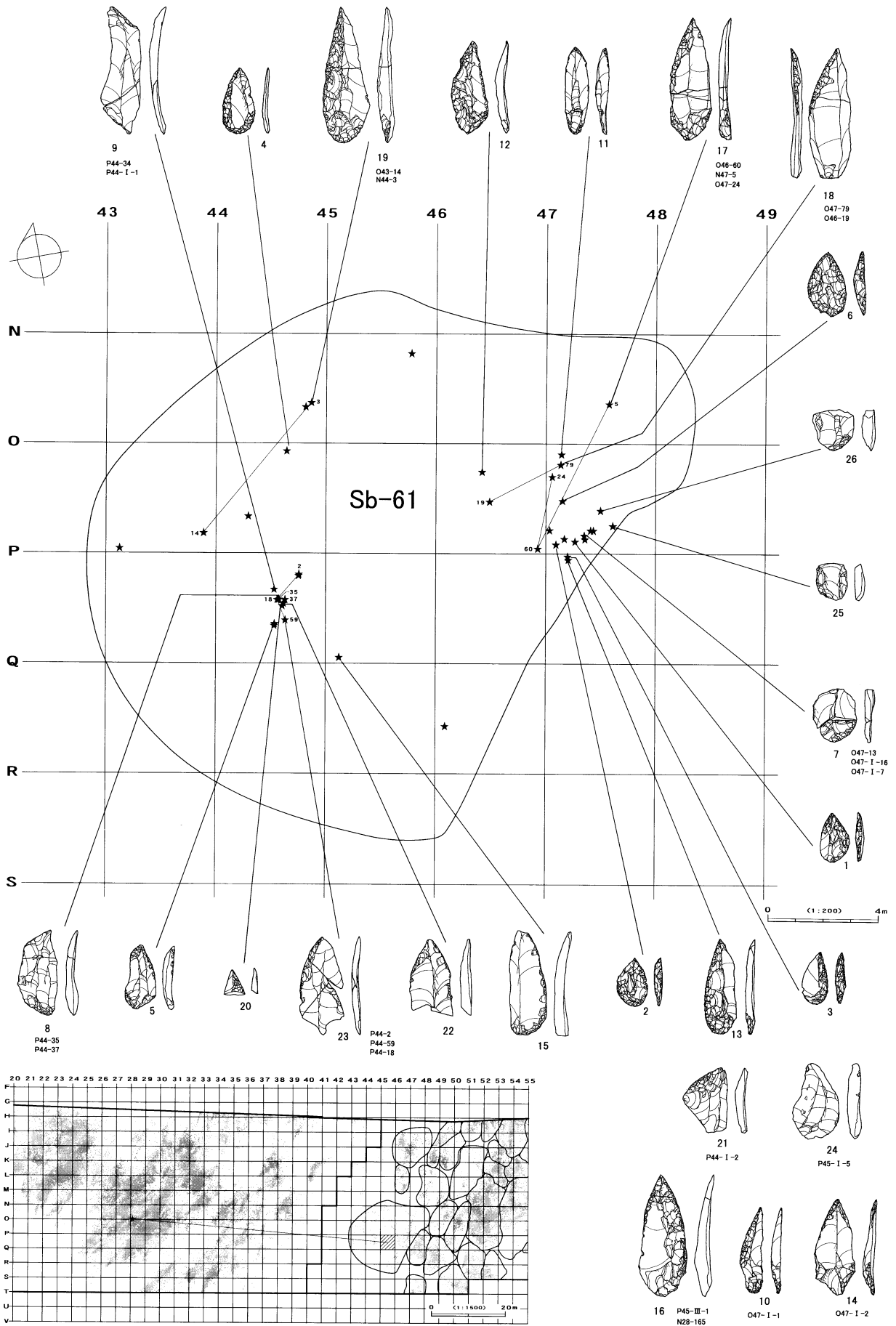
図IV-560 Sb-61の遺物(1)
