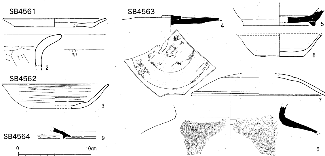
Fig.38 SB4561~4564出土土器実測図 (1/3)
