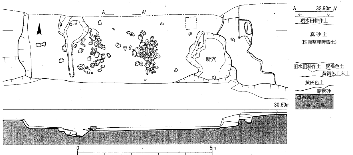
Fig.26 SX4565実測図 (1/80)
