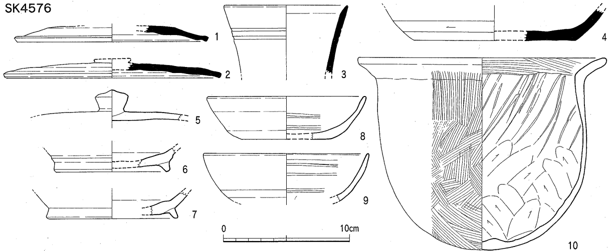
Fig.43 SK4576出土土器実測図 (1/3)
