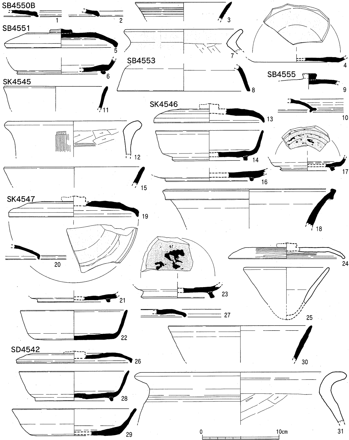
Fig.8 建物・土壇・溝出土土器実測図 (1/3)
