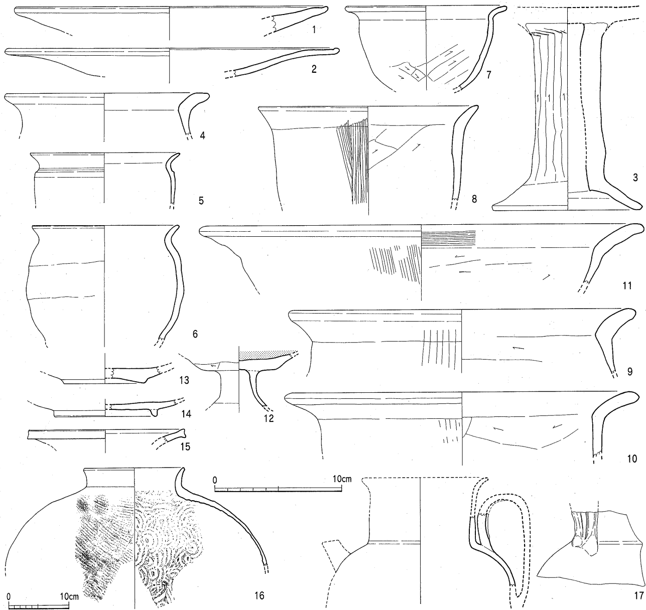
Fig.40 SK4573黒色土出土土器実測図 (1/3, 16:1/6)
