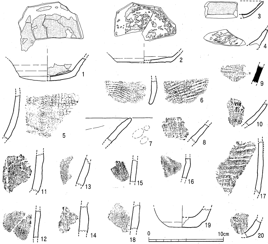
Fig.53 漆付着土器・製塩土器実測図 (1/3)
