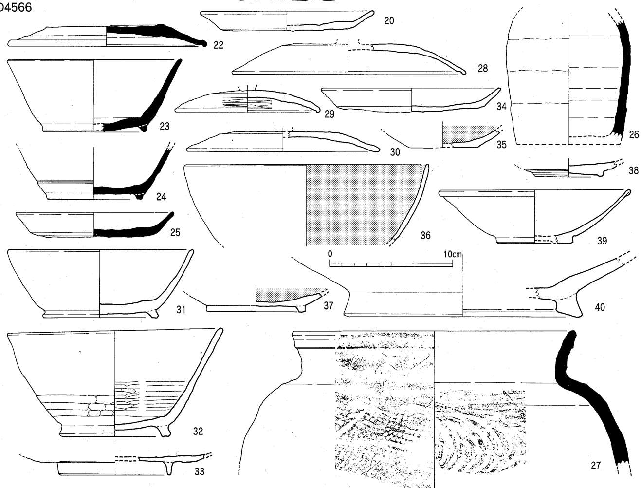
Fig.44 SD4566出土土器実測図 (1/3)
