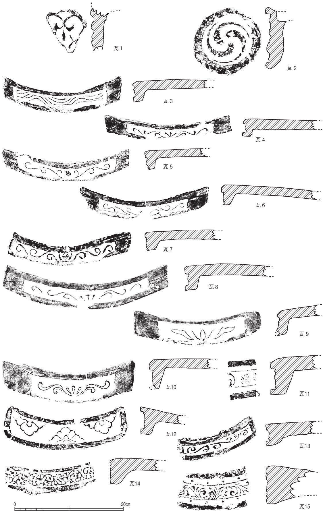
图37 軒瓦拓影·实测图 (1/4)
