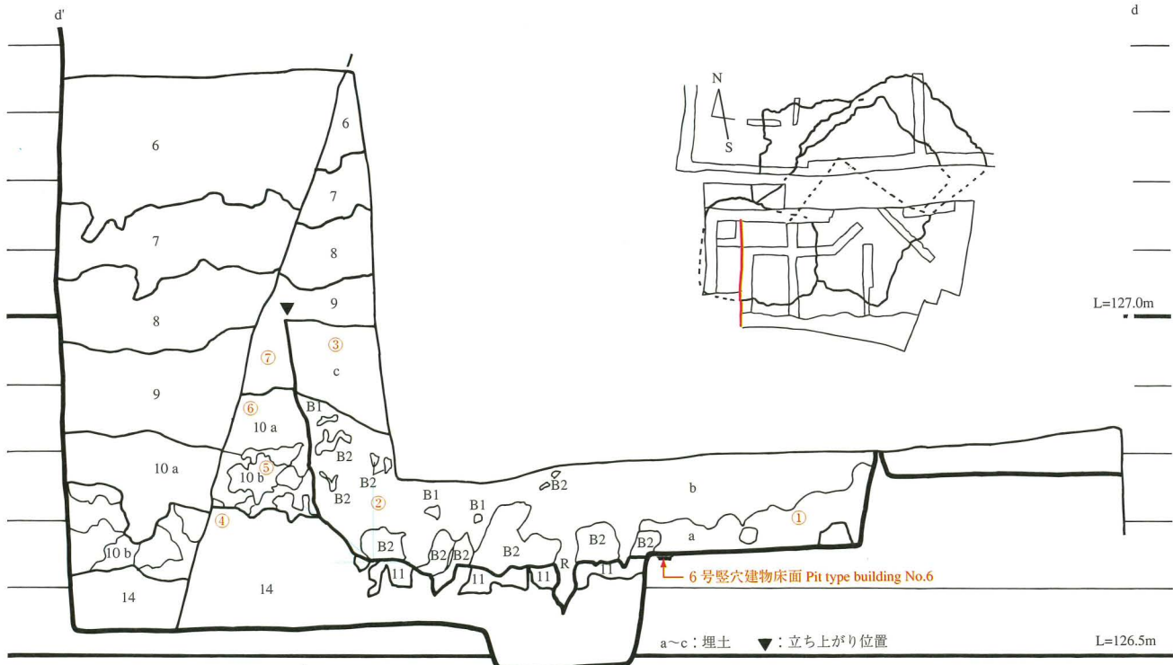
Fig.82 6号竖穴建物跡試掘溝L断面図(d-d')(S=1/10) Section d-d' of test trench L of pit type building No.6
