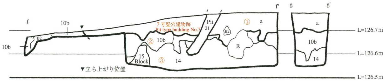
Fig.92 7号竖穴建物跡試掘溝E断面図(f-f', g-g') (1/10) Section f-f', g-g' of test trench E of pit type building No.7
