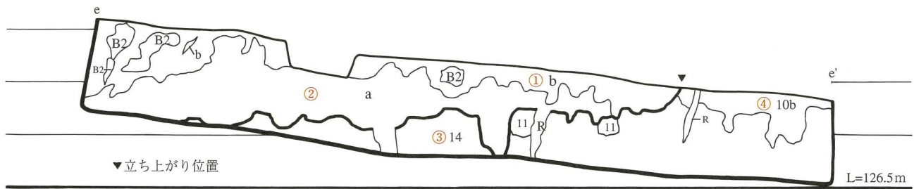
Fig.83 6号竖穴建物跡試掘溝H断面図(e-e' )(1/10) Section e-e' of test trench H of pit type building No.6
