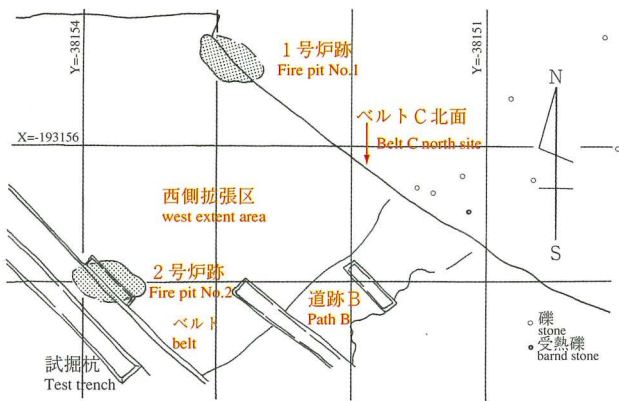
Fig.101 1号・2号炉跡, 受熱礫位置図(S=1/50) Position of fire pit No.1,2 and heated stones
