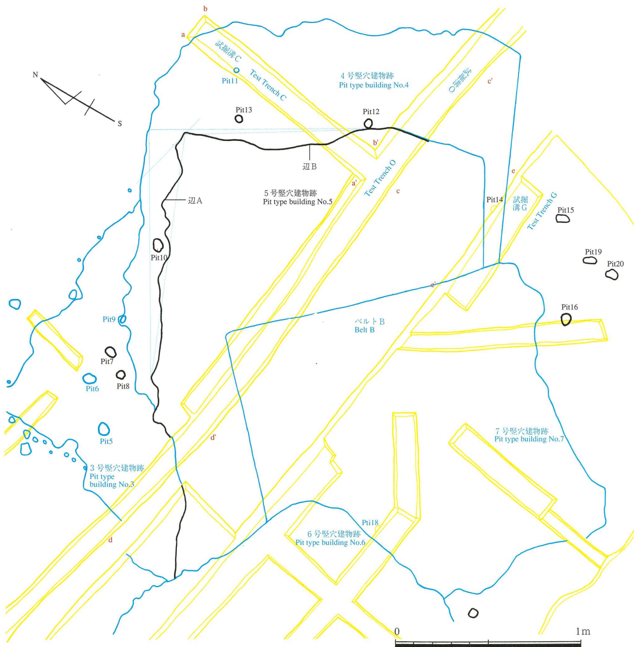
Fig.70 5号竖穴建物跡平面図(S=1/20) Plan of pit type building No.5
