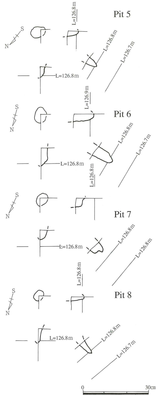
Fig97 竪穴建物跡周辺ピット平面図・断面図②(S=1/10) Plan and cross section of the pits with pit type building
