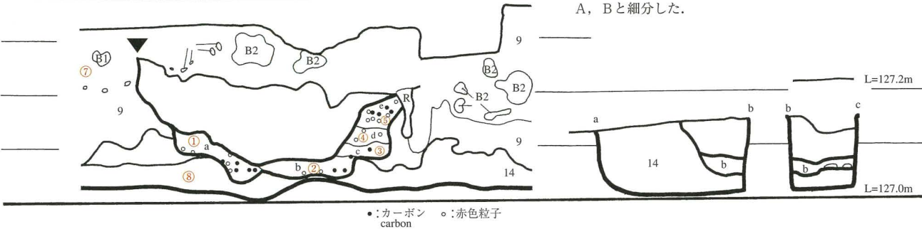
Fig.102 1号炉跡A平面・断面図(S=1/10) Plan and section of fire pit 'A' of No.1
