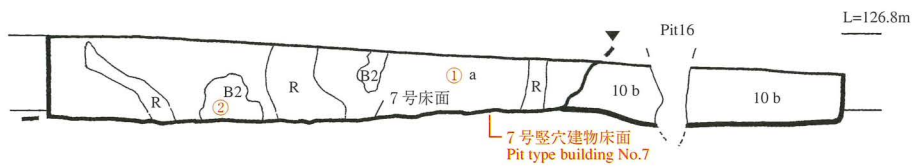
Fig.89 7号竖穴建物跡試掘溝D断面图(d-d') (1/10) Section d-d' of test trench D of pit type building No.7
