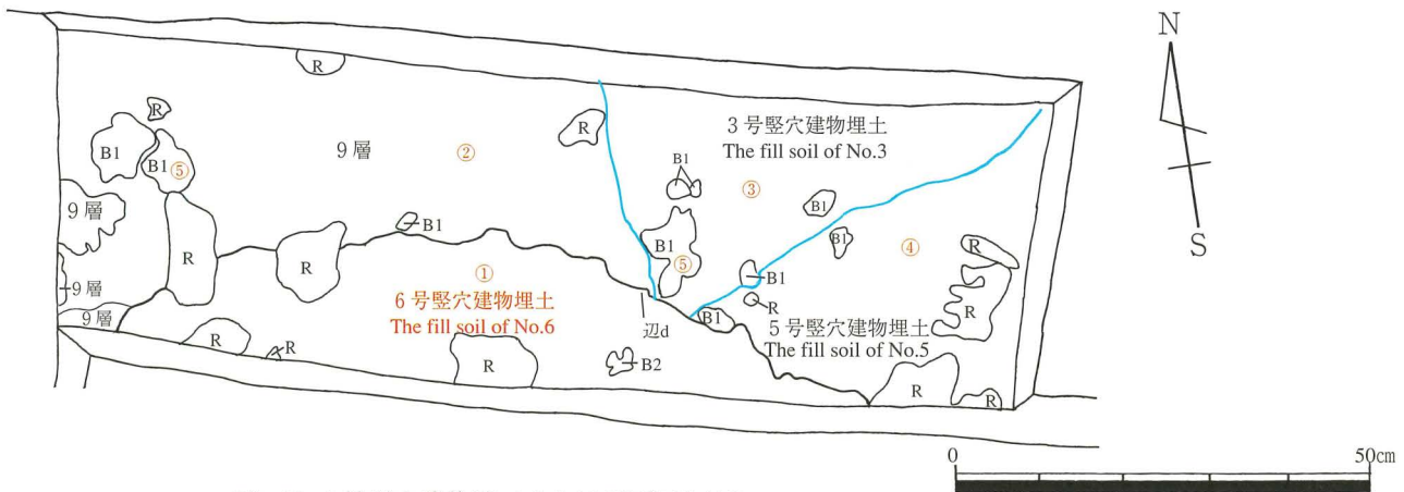
Fig.78 6号竪穴建物跡ベルトB平面図(1/10) Plan of the pit type building No.6 in Belt B
