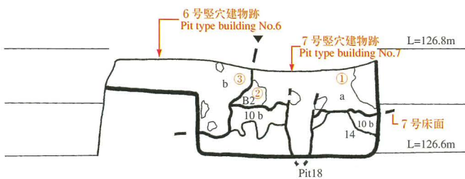
Fig.90 7号竖穴建物跡試掘溝K断面图(j-j') (1/10) Section j-j' of test trench K of pit type building No.7
