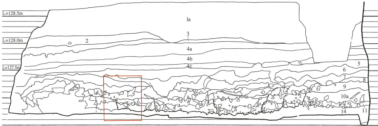
Fig.67 西側拡張区ベルトB北断面(1/40) North side section of Belt B in west extent area
