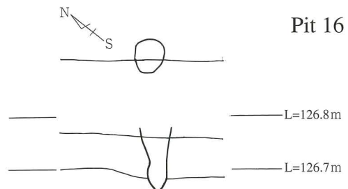
Fig.99 竪穴建物跡周辺ピット平面図・断面図④(S=1/10) Plan and cross section of the pits with pit type building
