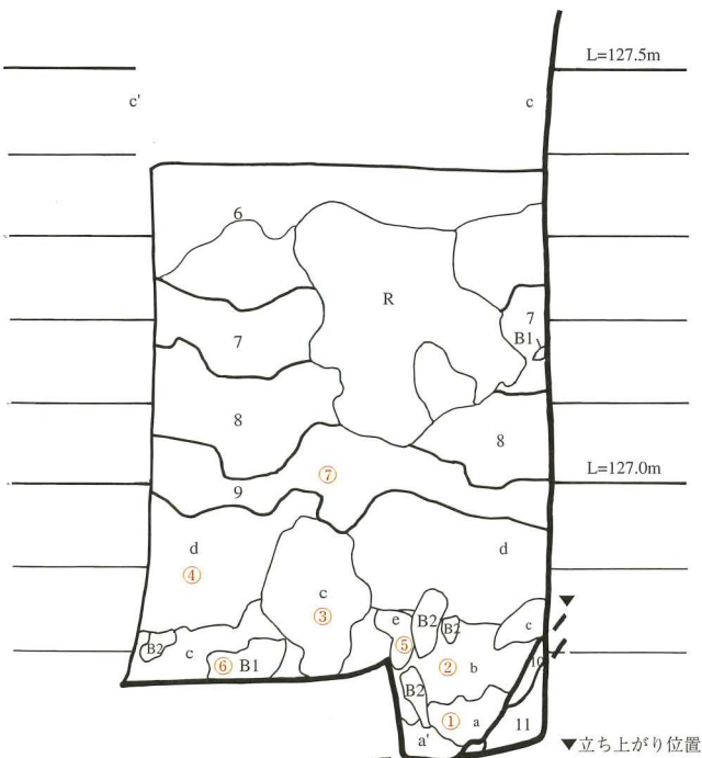
Fig.81 6号竖穴建物跡試掘溝J断面図(c-c')(S=1/10) Section c-c' in test trench L of pit type building No.6
