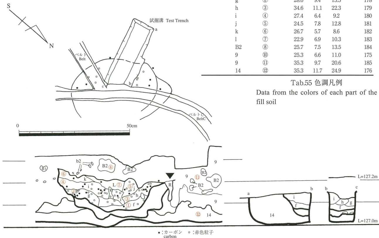
Fig.103 1号炉跡B平面・断面図(S=1/10) Plan and section of fire pit 'B' of No.1
