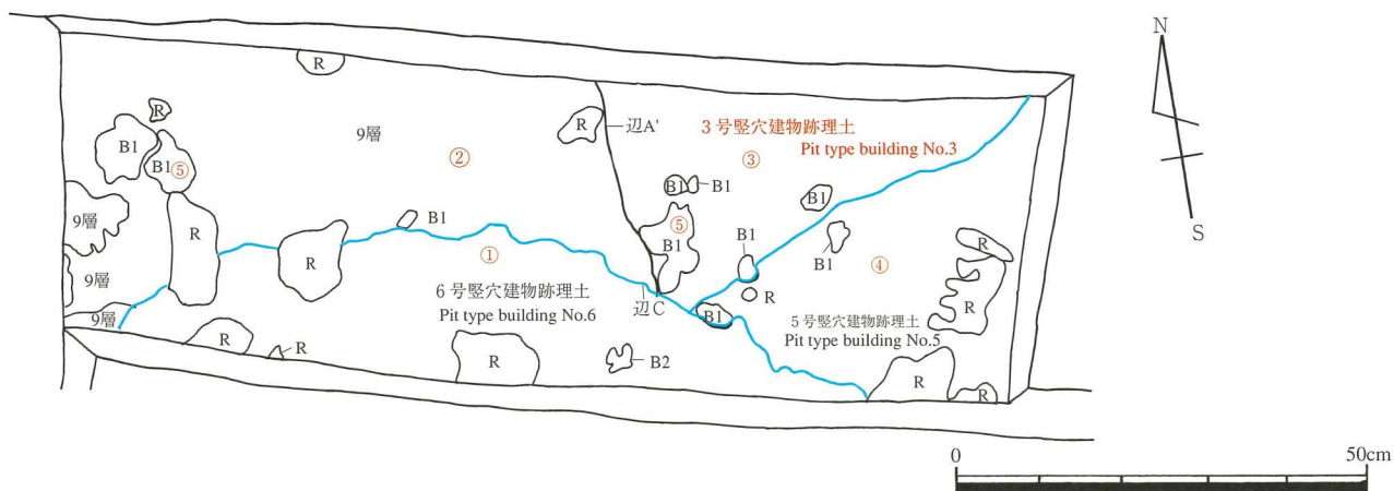
Fig.60 3号竖穴建物跡ベルトB平面図(1/10) Plane of pit type building No.3 in Belt B
