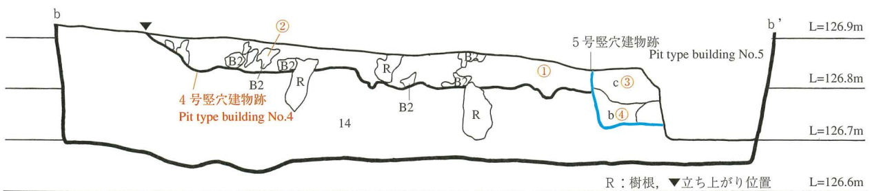
Fig.66 4号竖穴建物跡試掘溝C断面図(b-b') (1/10) Section b-b' of test trench C of pit type building No.4
