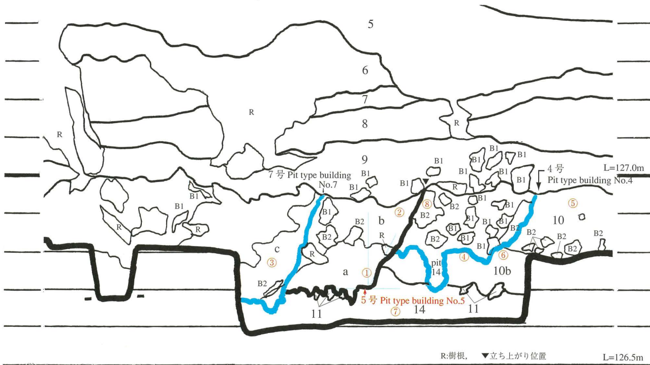
Fig.76 5号竖穴建物跡 試掘溝G断面図(e-e')(S=1/10) Section e-e' of test trench G of pit type building No.5
