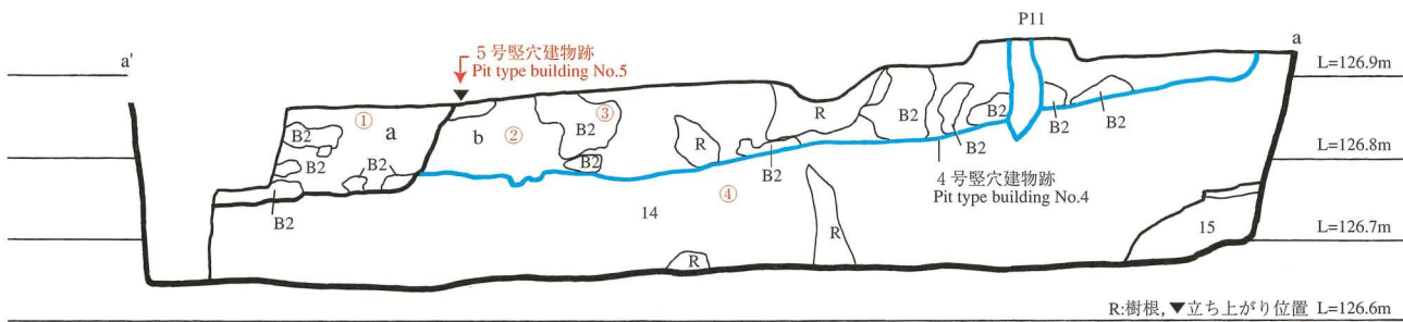
Fig.72 5号竖穴建物跡試掘溝C断面図(a-a') (1/10) Section a-a' of test trench C of pit type building No.5
