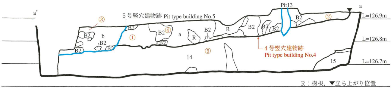
Fig.65 4号竖穴建物跡試掘溝C断面図(a-a') (1/10) Section a-a' of test trench C of pit type building No.4
