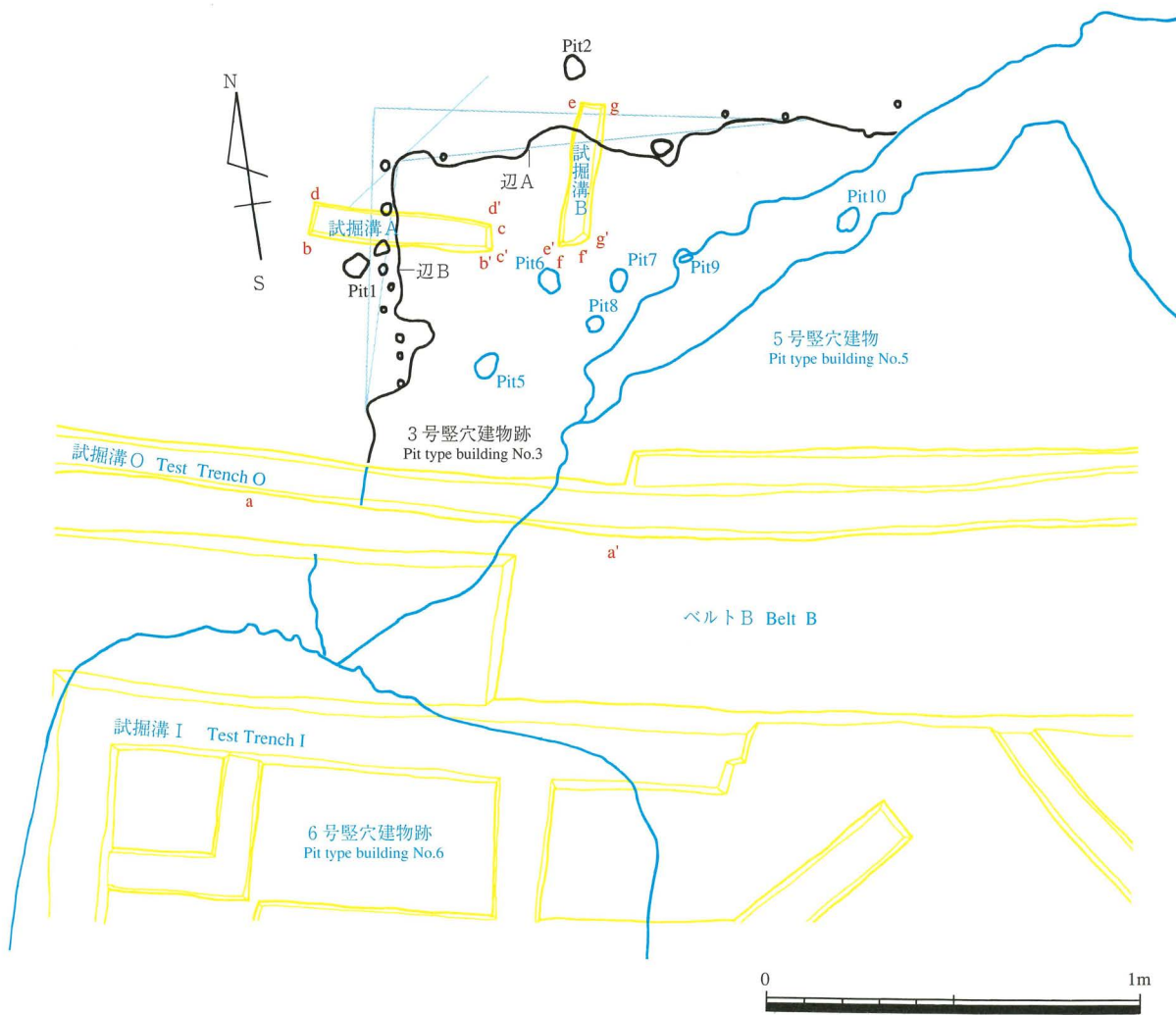
Fig.59 3号竖穴建物跡平面図(S=1/20) Plan of pit type building No.3
