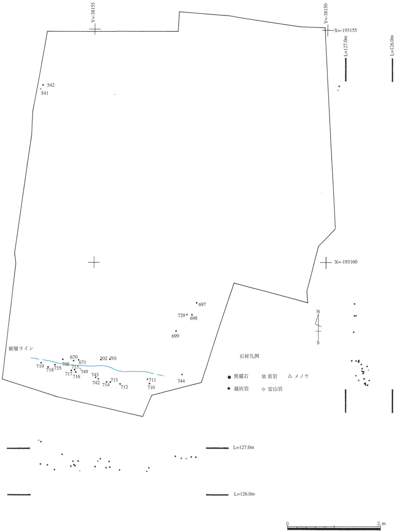
Fig.123 第10層出土遺物の石材別平面・垂直分布図(S=1/50) Plan and section map of the distribution of artifacts from the 10th layer by division of each of the materials
