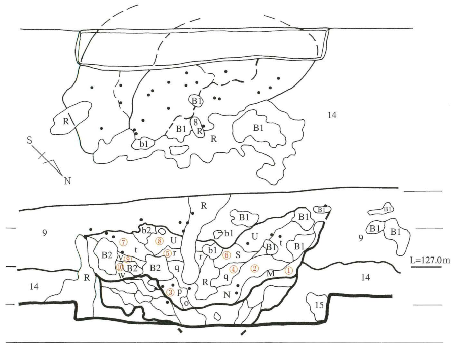
Fig.105 2号炉跡B平面・断面図(S=1/10) Plan and section of fire pit 'B' of No.2
