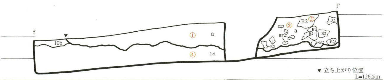
Fig.84 6号竖穴建物跡試掘溝H断面図(f-f' )(1/10) Section f-f' of test trench H of pit type building No.6
