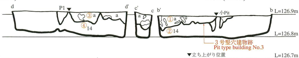
Fig.62 3号竖穴建物跡試掘溝A断面図(b-b', c-c', d-d') (1/10) Section b-b', c-c' and d-d' of test trench A of pit type building No.3
