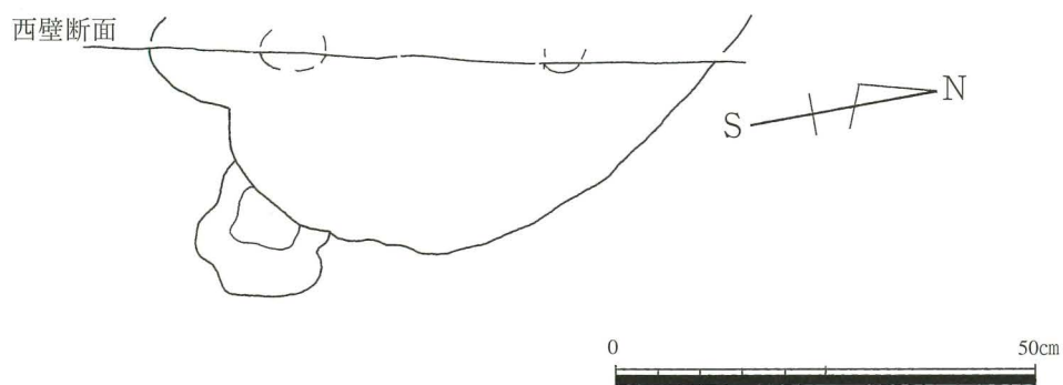
Fig.107 土坑平面図(S=1/10) Plan of earthen pit
