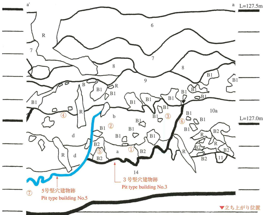
Fig.61 3号竖穴建物跡試掘溝O断面図(a-a') (S=1/10) Section a-a' of test trench O of pit type building No.3
