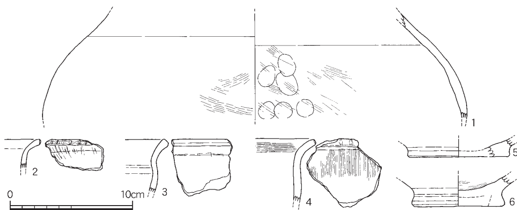
Fig.17 SK07出土遺物実測図 (S=1/3)
