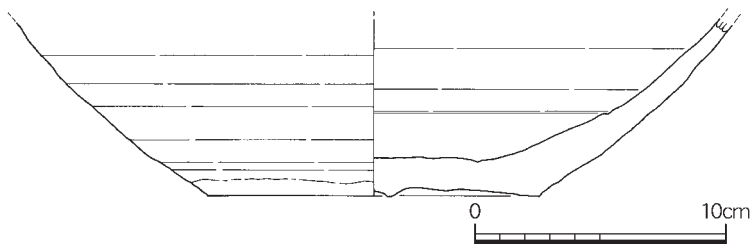
Fig.40 SB100出土遺物実測図 (S=1/3)
