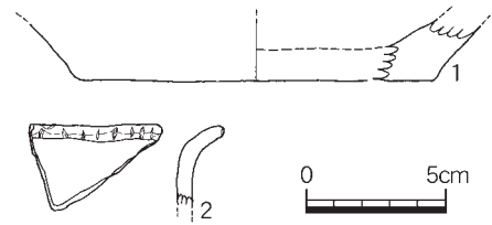
Fig.23 SP96出土遺物実測図 (S=1/2・S=1/3)
