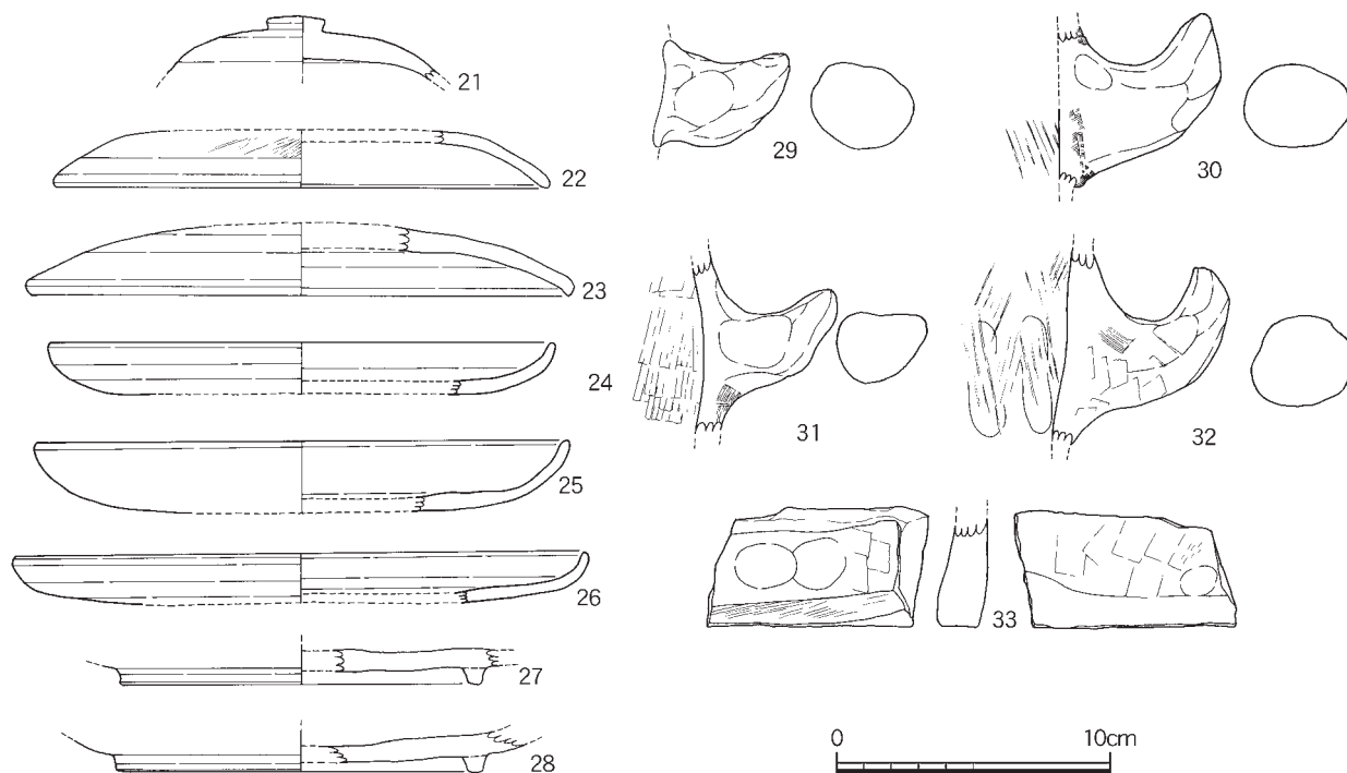
Fig.27 SD09出土遺物実測図② (S=1/3)
