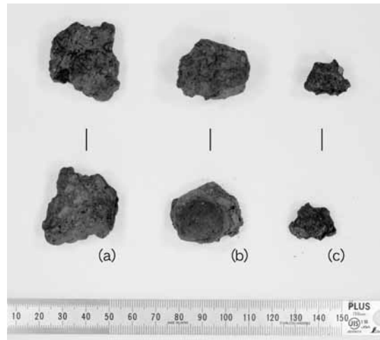
Ph.12 SD09出土炉壁・鉄滓
