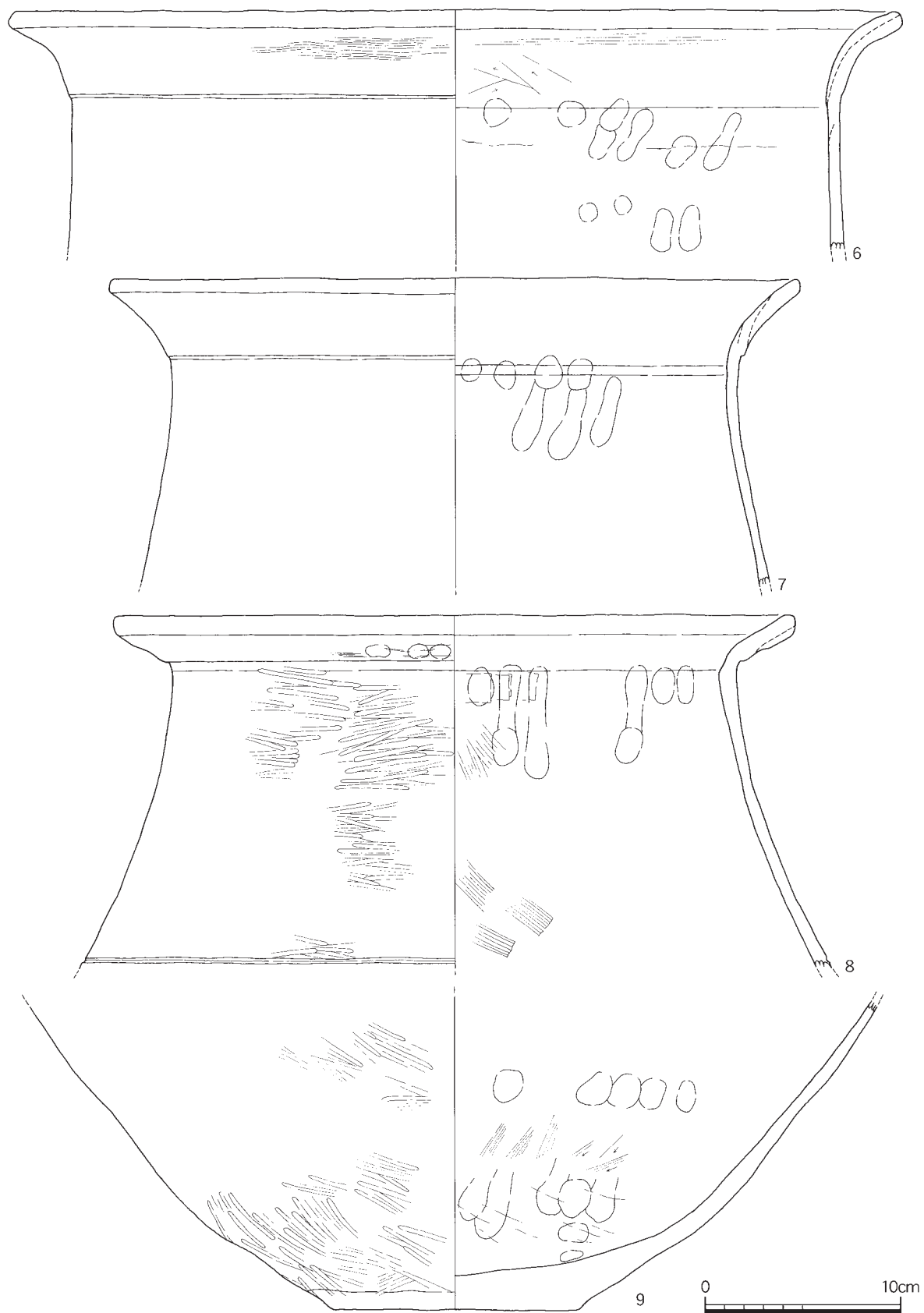
Fig.11 SK02出土遺物実測図③ (S=1/3)
