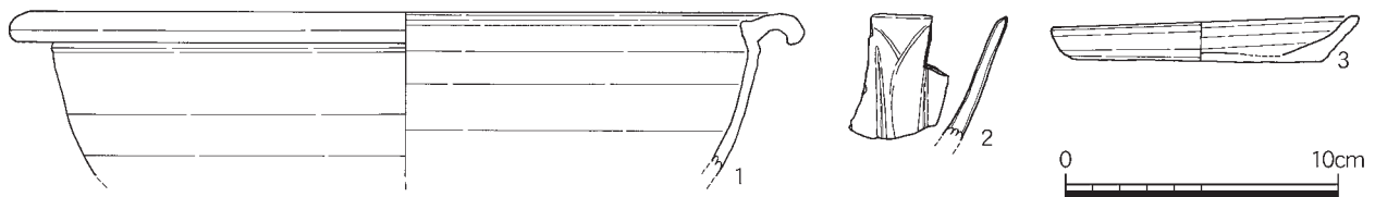
Fig.33 SK46出土遺物実測図 (S=1/3)
