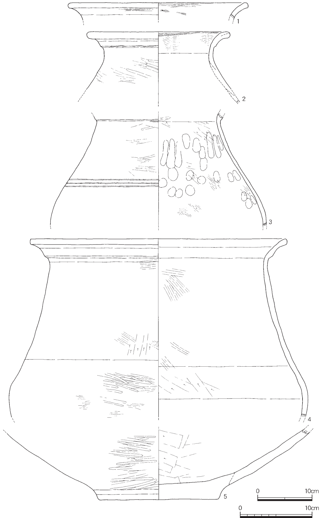
Fig.10 SK02出土遺物実測図② (S=1/3・1/4)
