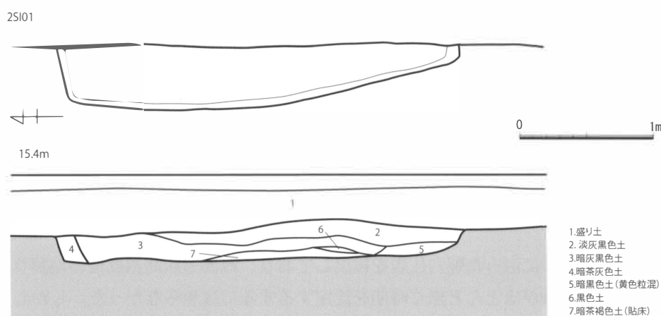
Fig.3 2SI01 遺構実測図 (1/40)
