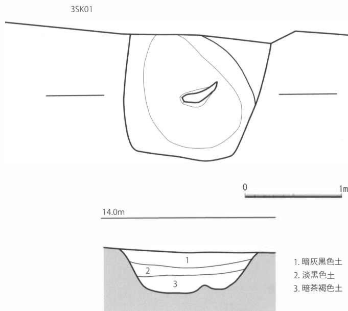
Fig.8 3SK01 遺構実測図 (1/40)
