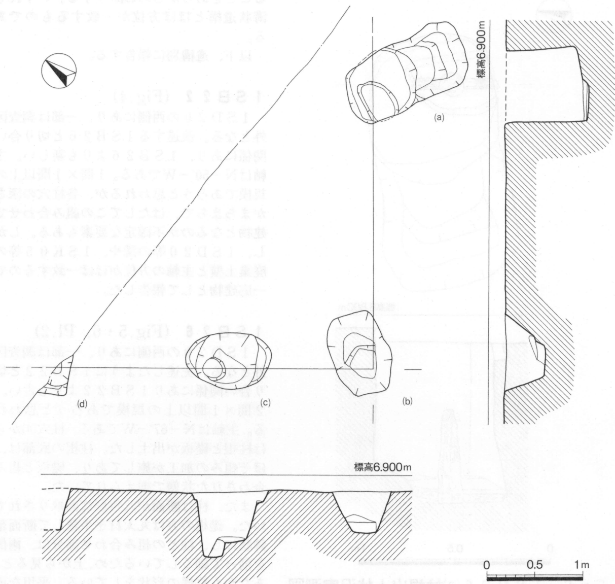
Fig.5 1SB26実測図(1/40)
