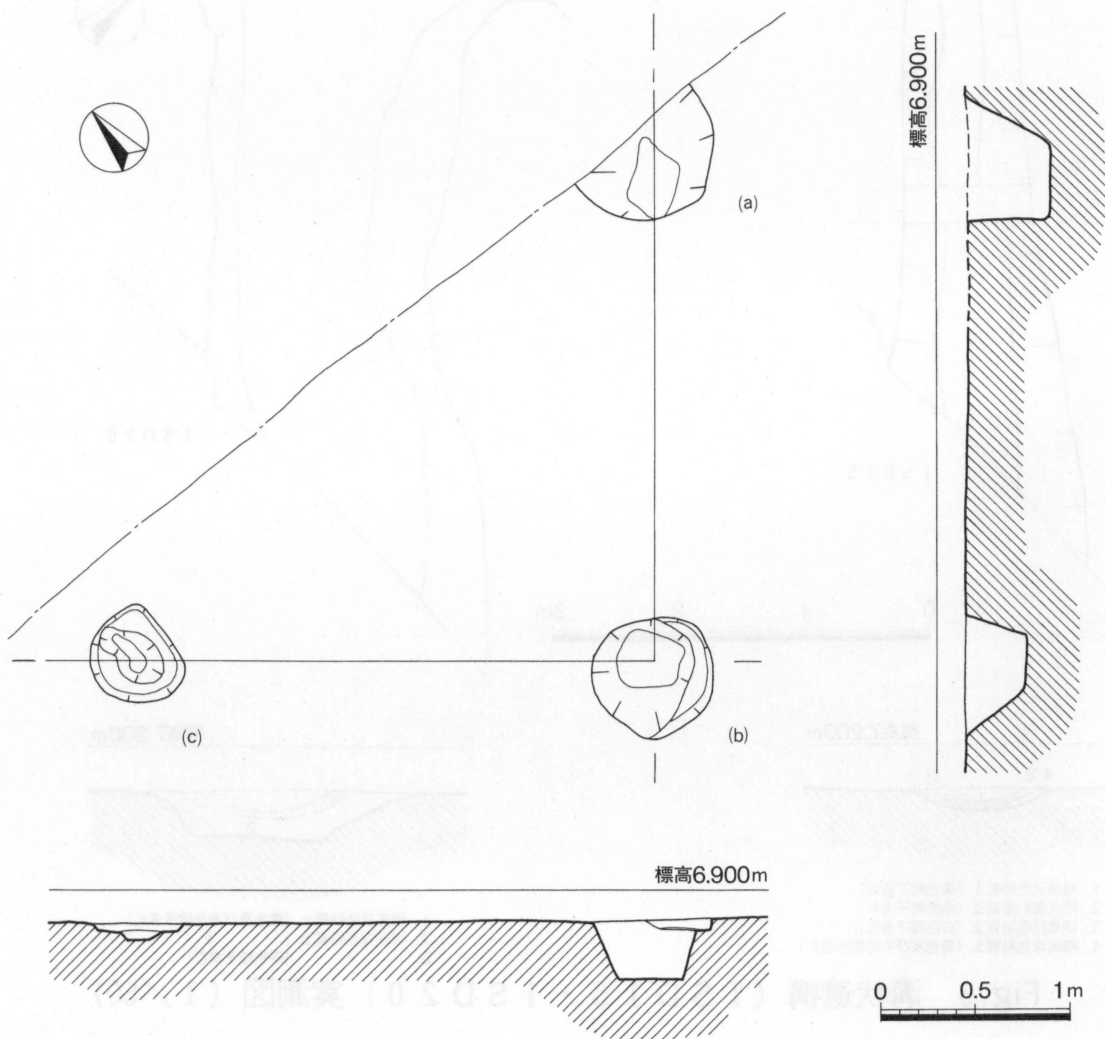
Fig.4 1SB22実測図(1/40)
