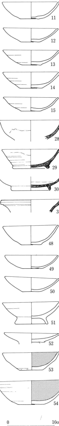
259图 ISD 1 (HSD 6), ISD 1-1·3·4 出土土器实测图 (1:4)
