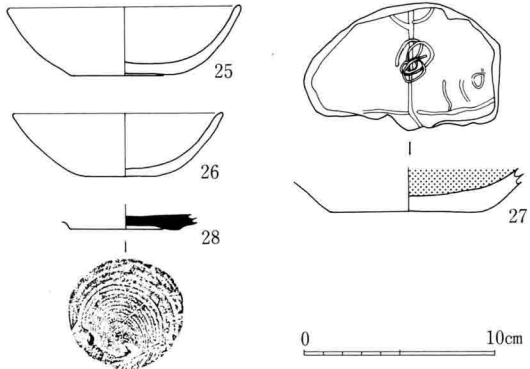
221图 LS B82~84·86·88·90·91·94·99出土土器实测图(1:4)
