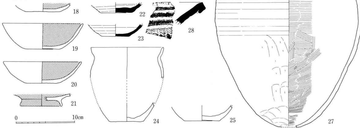
20図 AS B67・70~72出土土器実測図(1:4)
