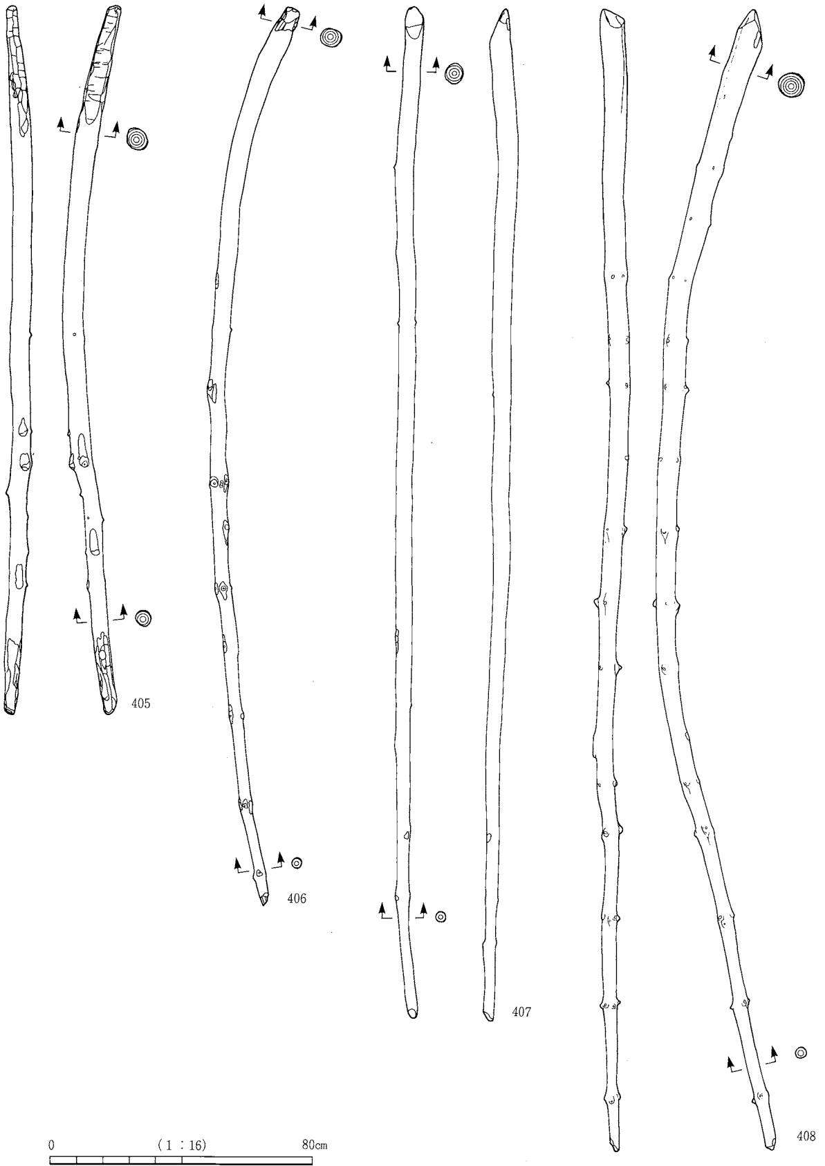
垂木 3
