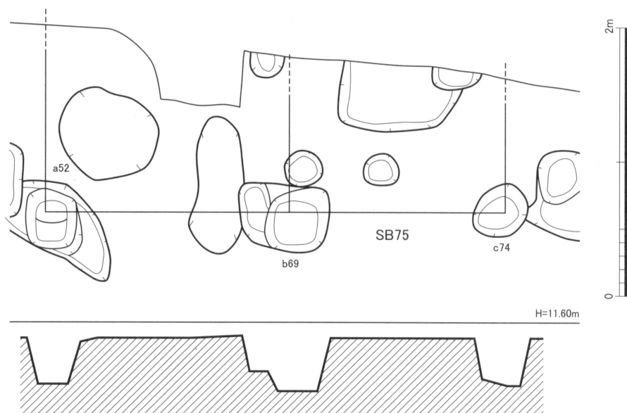
Fig.11 SB75実測図 (1/40)
