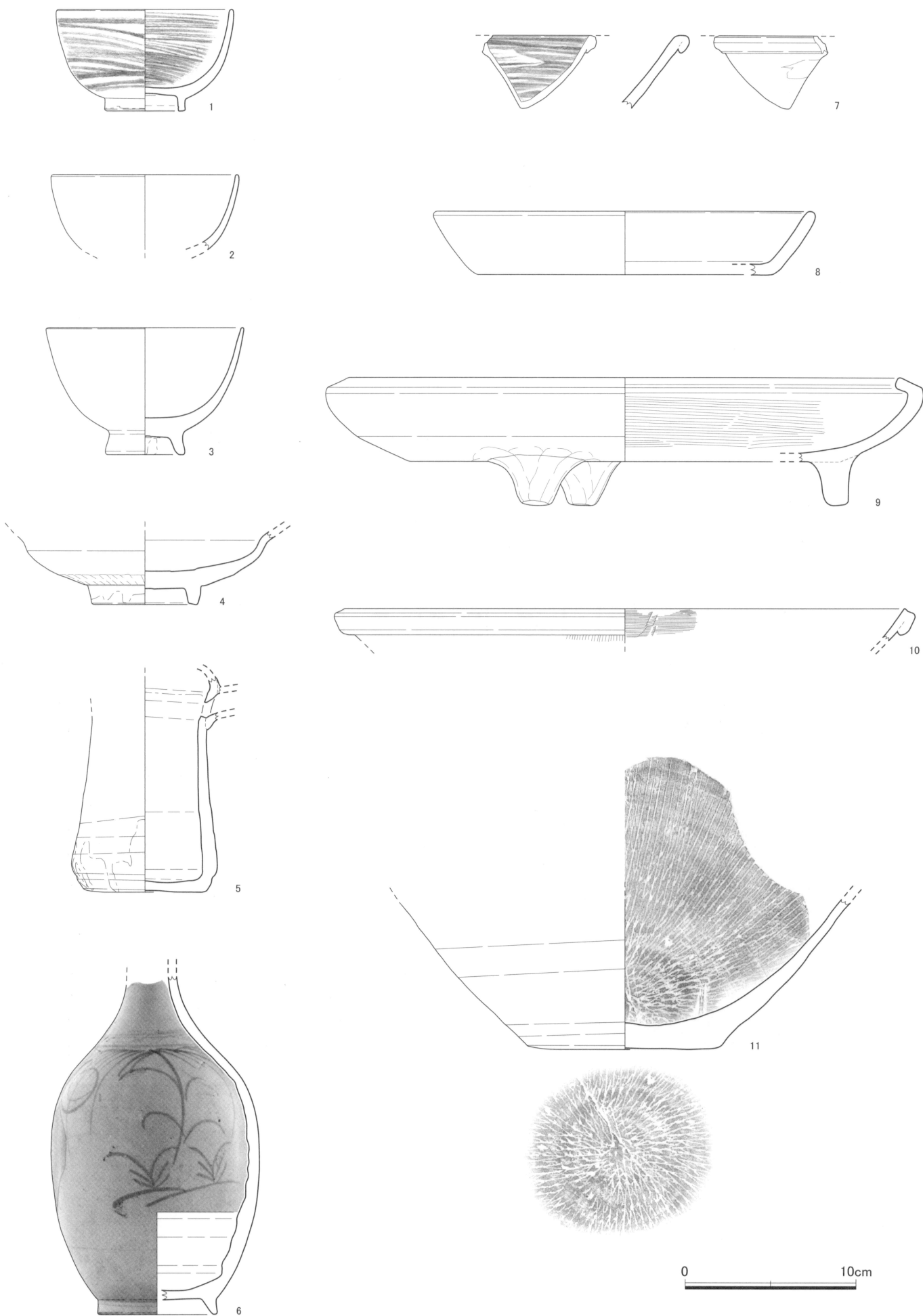
Fig.14 出土遺物実測図1 (1/3)
