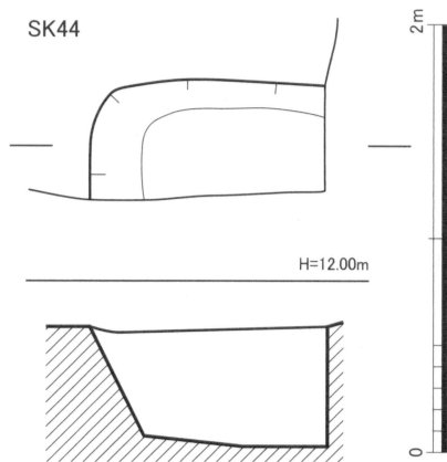
Fig.10 SK44実測図 (1/40)
