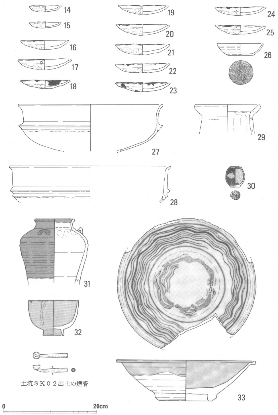
図6 出土遺物実測図2 (S=1/4)
