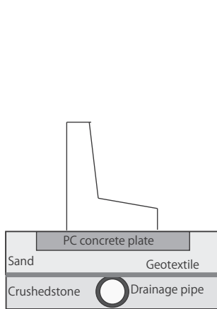
Fig. 16: Unwoven textile application example
