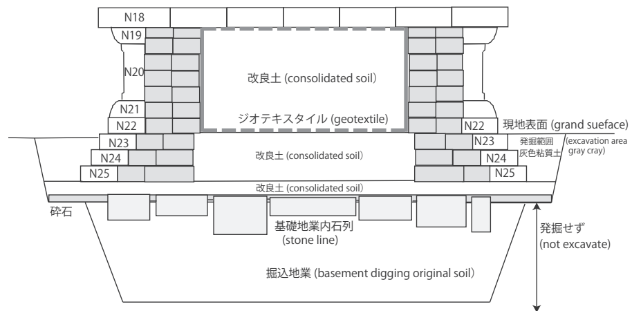
Fig. 17: Covering the foundation material with unwoven fabric
