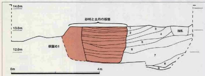
大仏殿礎石下根固め遺構の断面図 The cross section of the mark of the base under the foundation stone of Daibutsuden.
