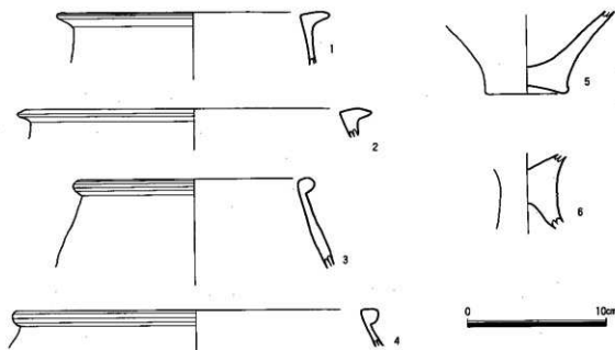
Fig.30 出土遺物実測図(1/3)
