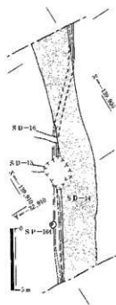
fig.10 SD-17平面図
