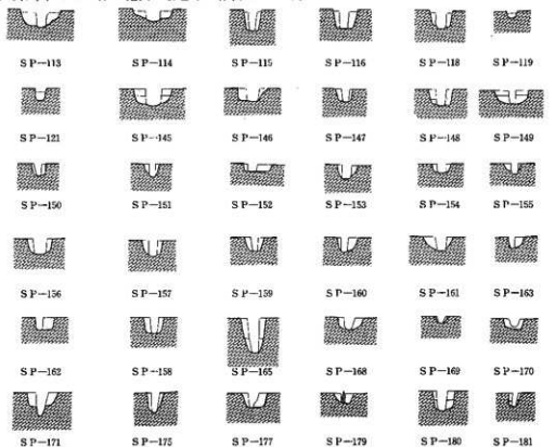
fig.23 柱穴断面図(1)
