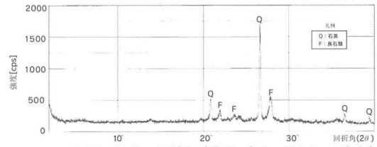
図4.2-2 X線回折図 (No.210 壁土)
