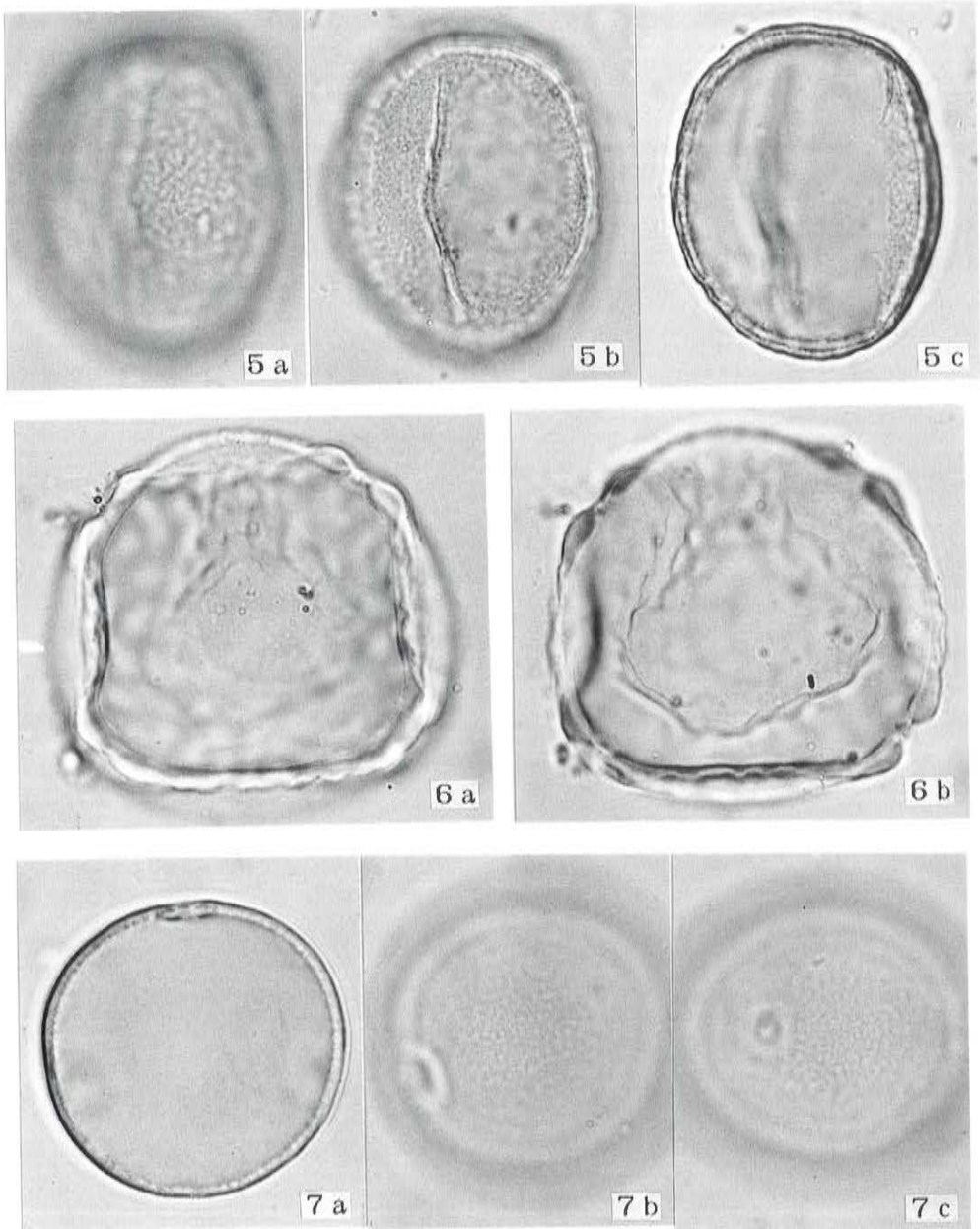
5 コナラ属コナラ亜属, No.7, PAL. MY 552 (x1,130)
