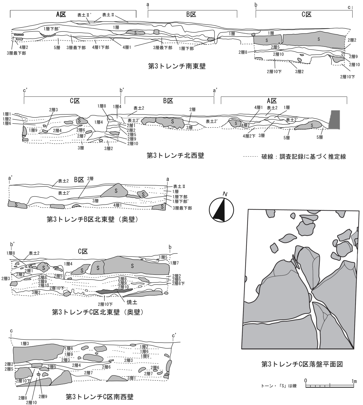
図2.7 第3トレンチセクション図とC区落盤平面図(右下)(S=1/40) Figure 2.7 The stratigraphic section of the 3rd trench and rock falls at the C grid.
