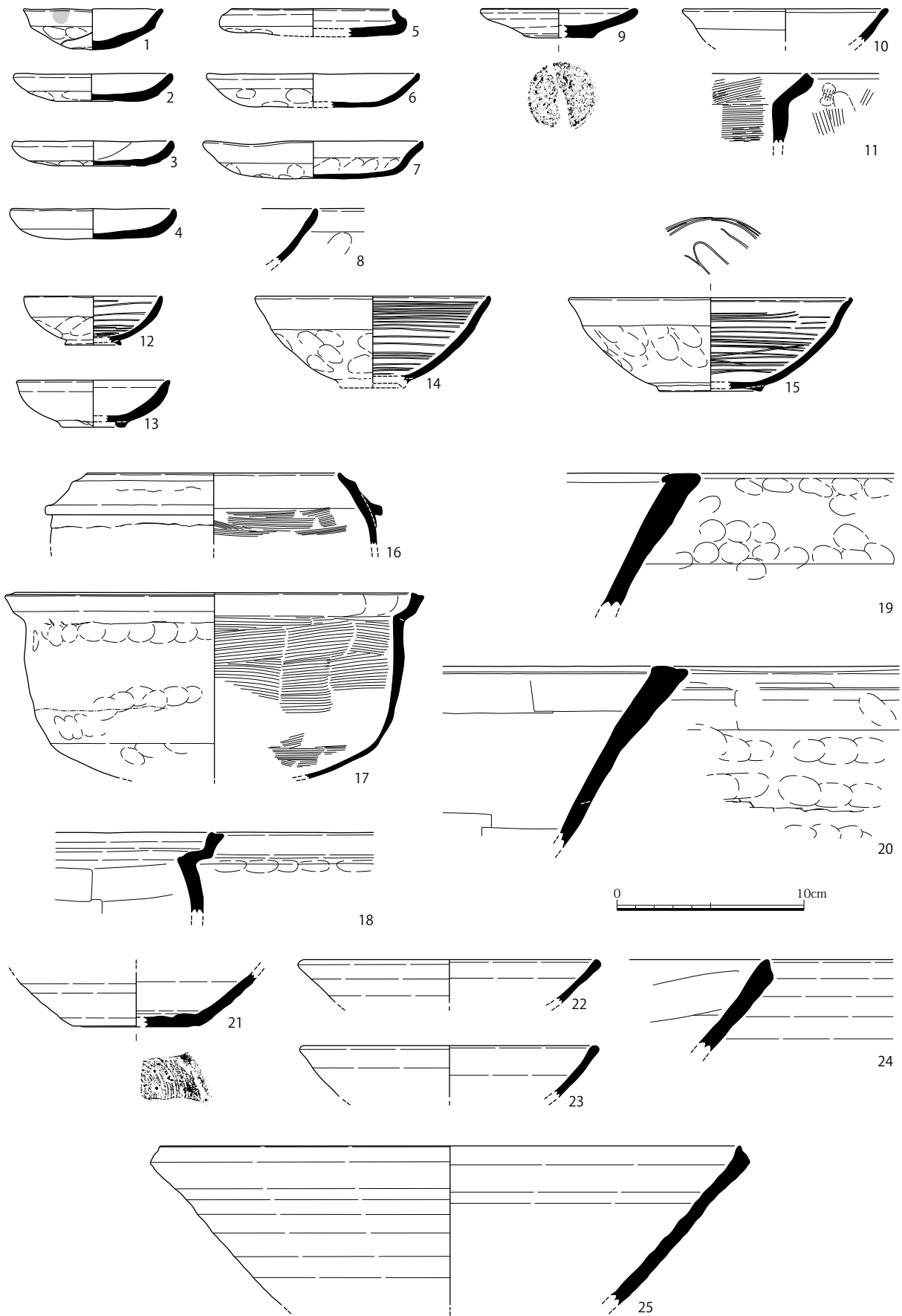
図19 整地土1出土遺物実測図(1) (S=1/3)
